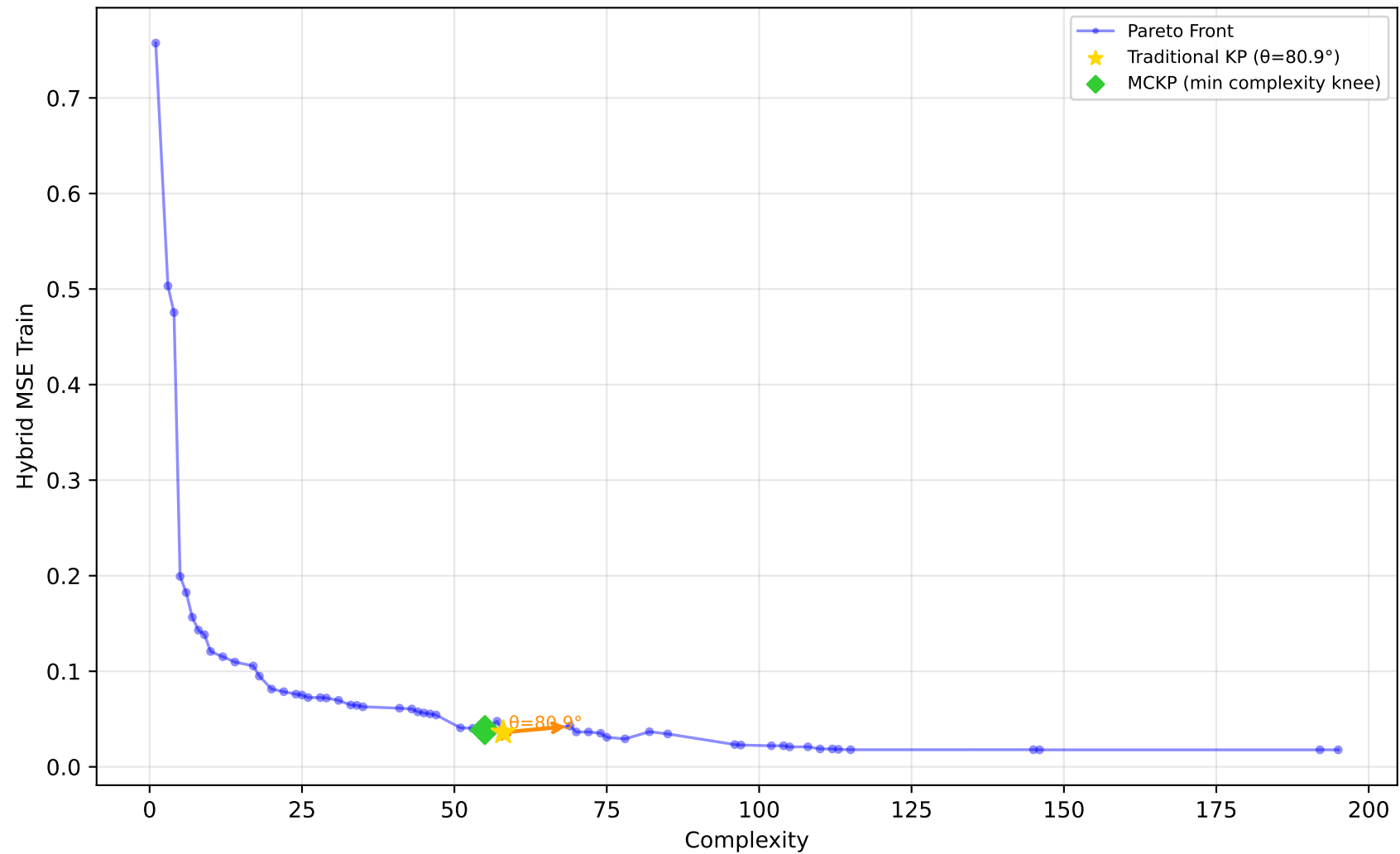
1096_FacultySalaries - Run 23 - MVP - Hybrid MSE Train \lambda_1=0.10 , \lambda_2=0.00 , \lambda_3=0.00 | Difficulty: 1.00 | Method: hmr
