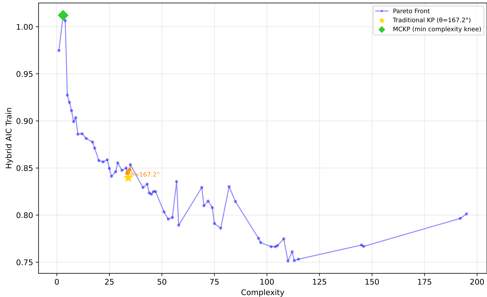
1096_FacultySalaries - Run 23 - SVP - Hybrid AIC Train \lambda_1=1.00 , \lambda_2=0.00 , \lambda_3=0.00 | Difficulty: 1.00 | Method: hmr
