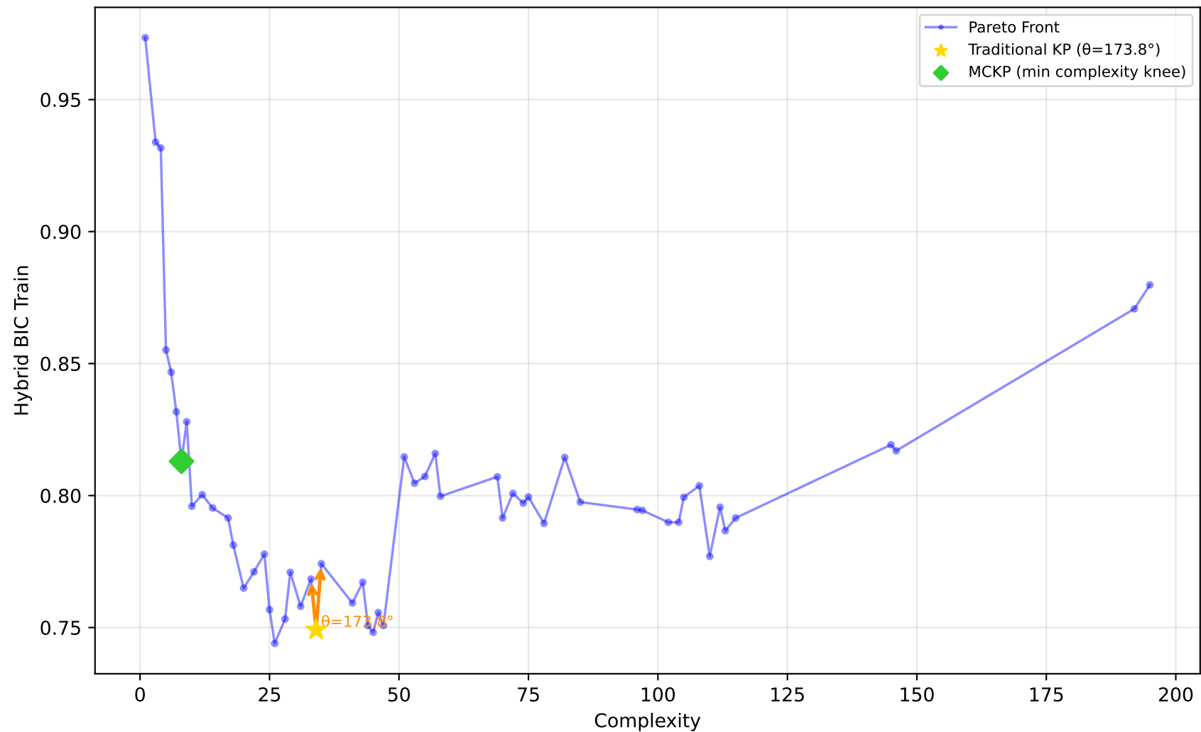
1096_FacultySalaries - Run 23 - SVP - Hybrid BIC Train \lambda_1=0.00 , \lambda_2=0.90 , \lambda_3=0.00 | Difficulty: 1.00 | Method: hmr
