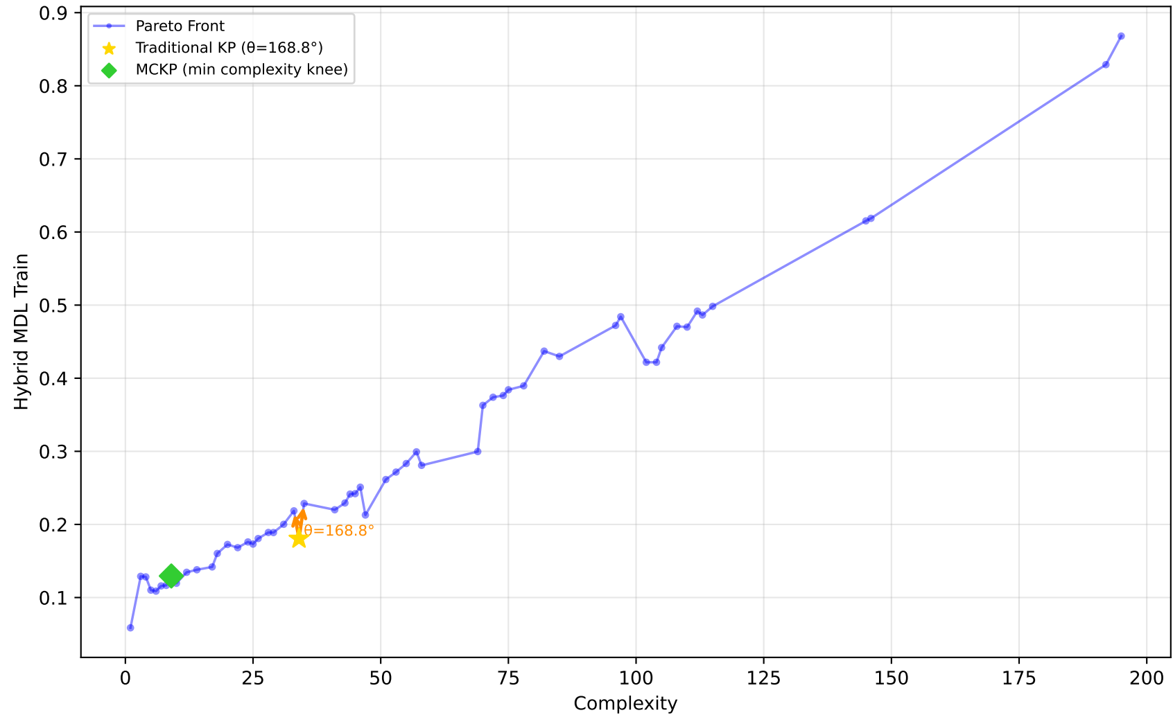
1096_FacultySalaries - Run 23 - SVP - Hybrid MDL Train \lambda_1=1.00, \lambda_2=0.00, \lambda_3=0.00 | Difficulty: 1.00 | Method: hmr
