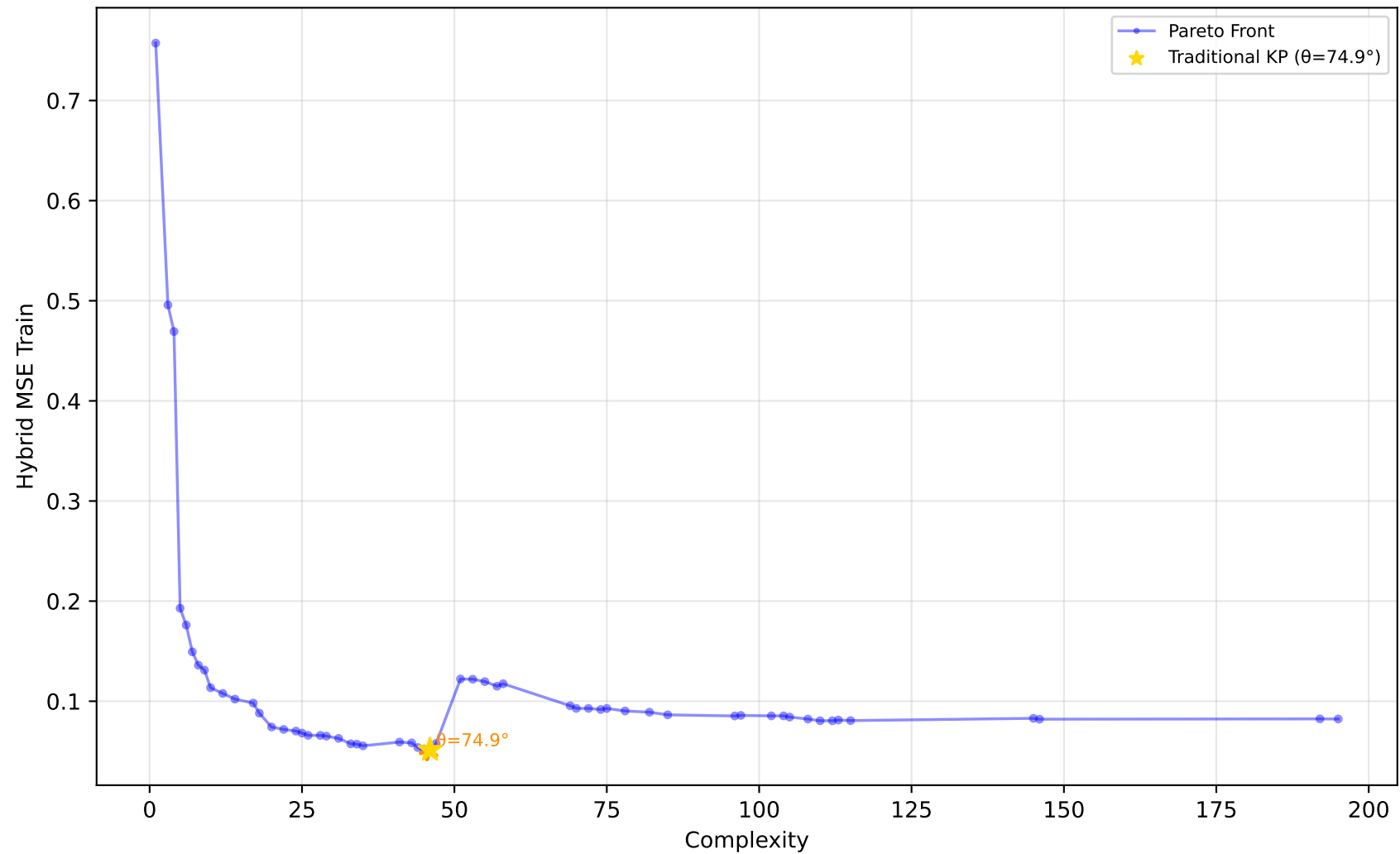
1096_FacultySalaries - Run 23 - SVP - Hybrid MSE Train \lambda_1=0.00, \lambda_2=0.90, \lambda_3=0.00 | Difficulty: 1.00 | Method: hmr
