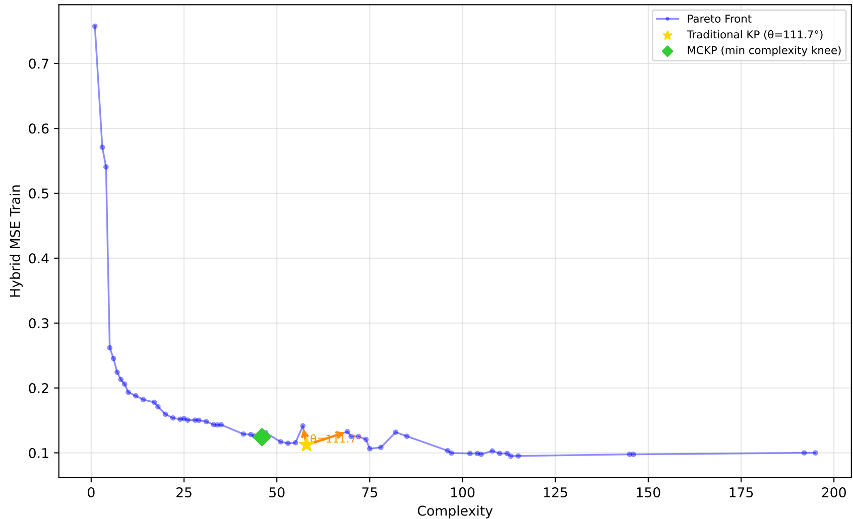
1096_FacultySalaries - Run 23 - SVP - Hybrid MSE Train \lambda_1=1.00, \lambda_2=0.00, \lambda_3=0.00 | Difficulty: 1.00 | Method: hmr
