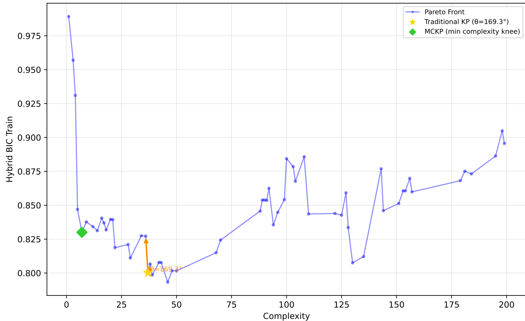
1096_FacultySalaries - Run 24 - MVP - Hybrid BIC Train \lambda_1=0.10 , \lambda_2=0.00 , \lambda_3=0.00 | Difficulty: 0.58 | Method: mckp
