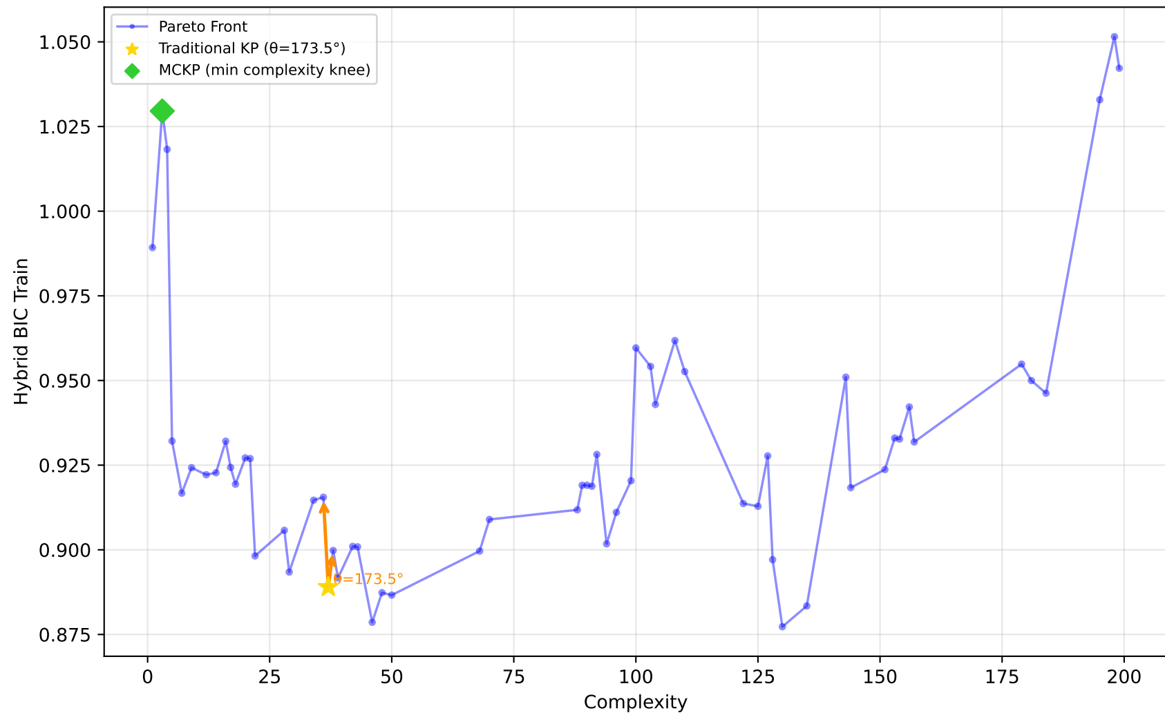
1096_FacultySalaries - Run 24 - MVP - Hybrid BIC Train \lambda_1=1.00 , \lambda_2=0.00 , \lambda_3=0.00 | Difficulty: 0.58 | Method: mckp
