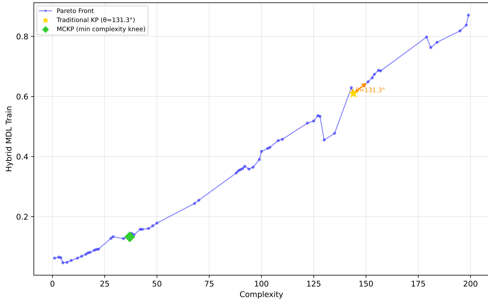
1096_FacultySalaries - Run 24 - MVP - Hybrid MDL Train \lambda_1=0.10, \lambda_2=0.00, \lambda_3=0.00 | Difficulty: 0.58 | Method: mckp
