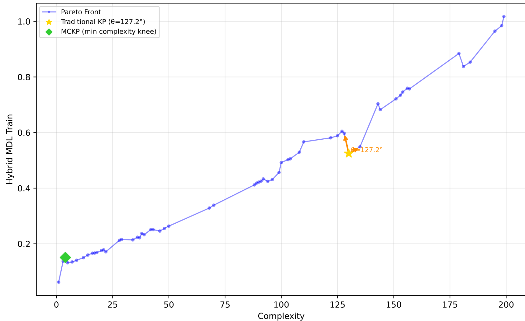
1096_FacultySalaries - Run 24 - MVP - Hybrid MDL Train \lambda_1=1.00, \lambda_2=0.00, \lambda_3=0.00 | Difficulty: 0.58 | Method: mckp
