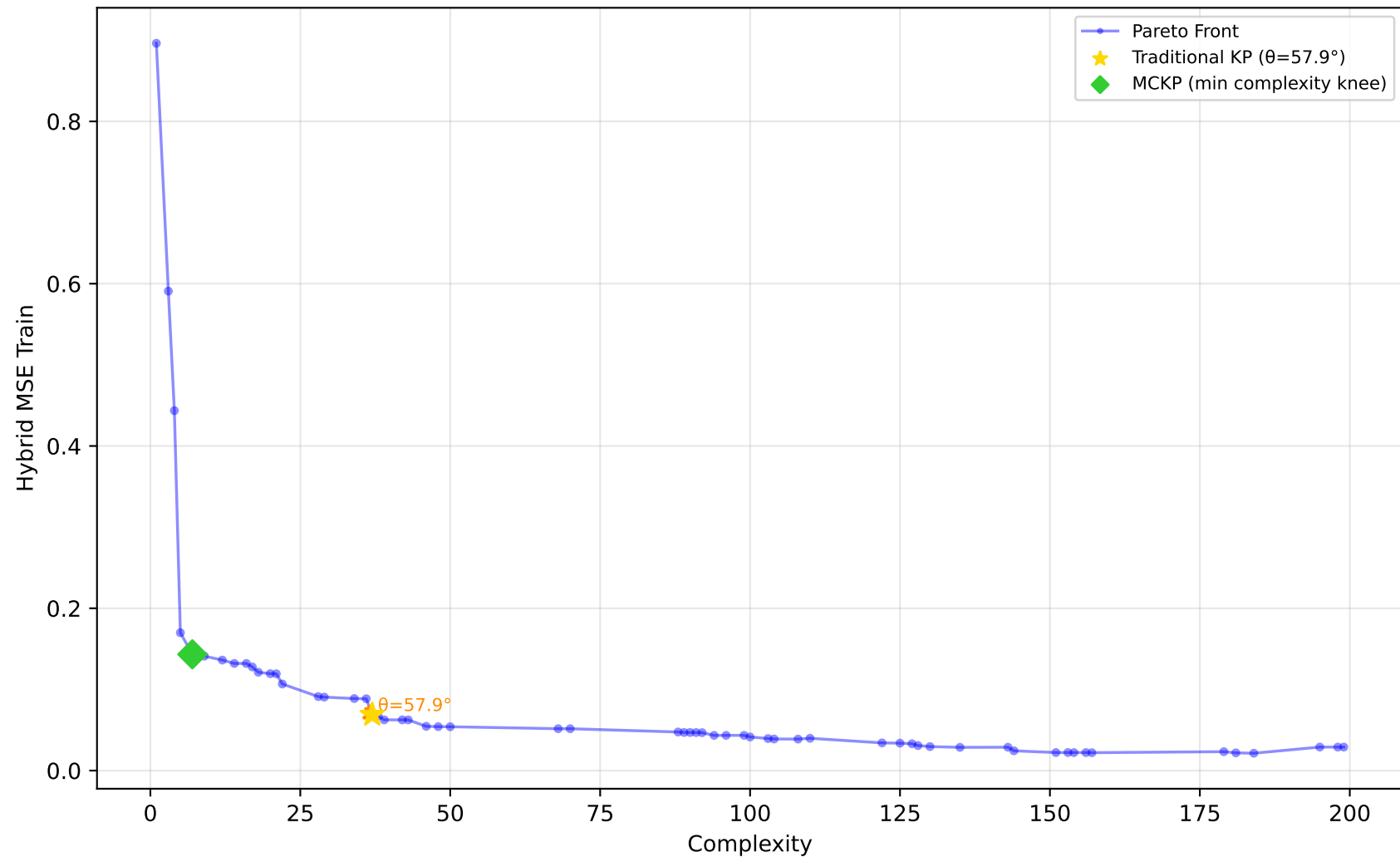
1096_FacultySalaries - Run 24 - MVP - Hybrid MSE Train \lambda_1=0.10, \lambda_2=0.00, \lambda_3=0.00 | Difficulty: 0.58 | Method: mckp
