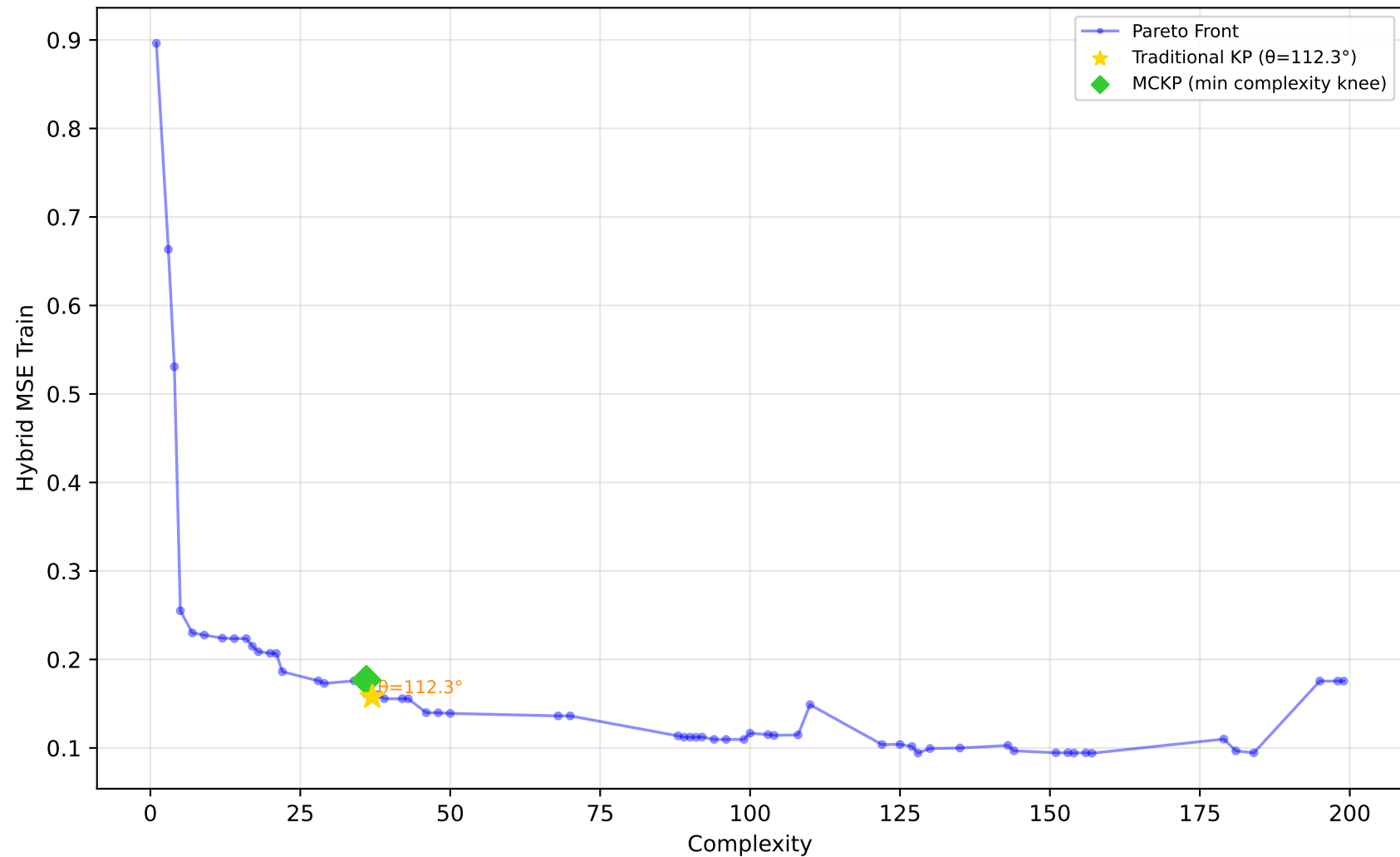
1096_FacultySalaries - Run 24 - MVP - Hybrid MSE Train \lambda_1=1.00 , \lambda_2=0.00 , \lambda_3=0.00 | Difficulty: 0.58 | Method: mckp
