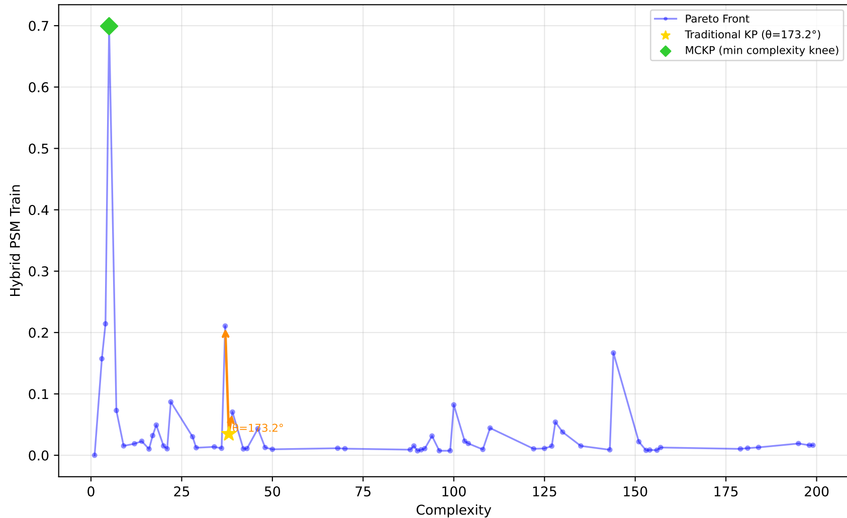
1096_FacultySalaries - Run 24 - MVP - Hybrid PSM Train \lambda_1=0.10, \lambda_2=0.00, \lambda_3=0.00 | Difficulty: 0.58 | Method: mckp
