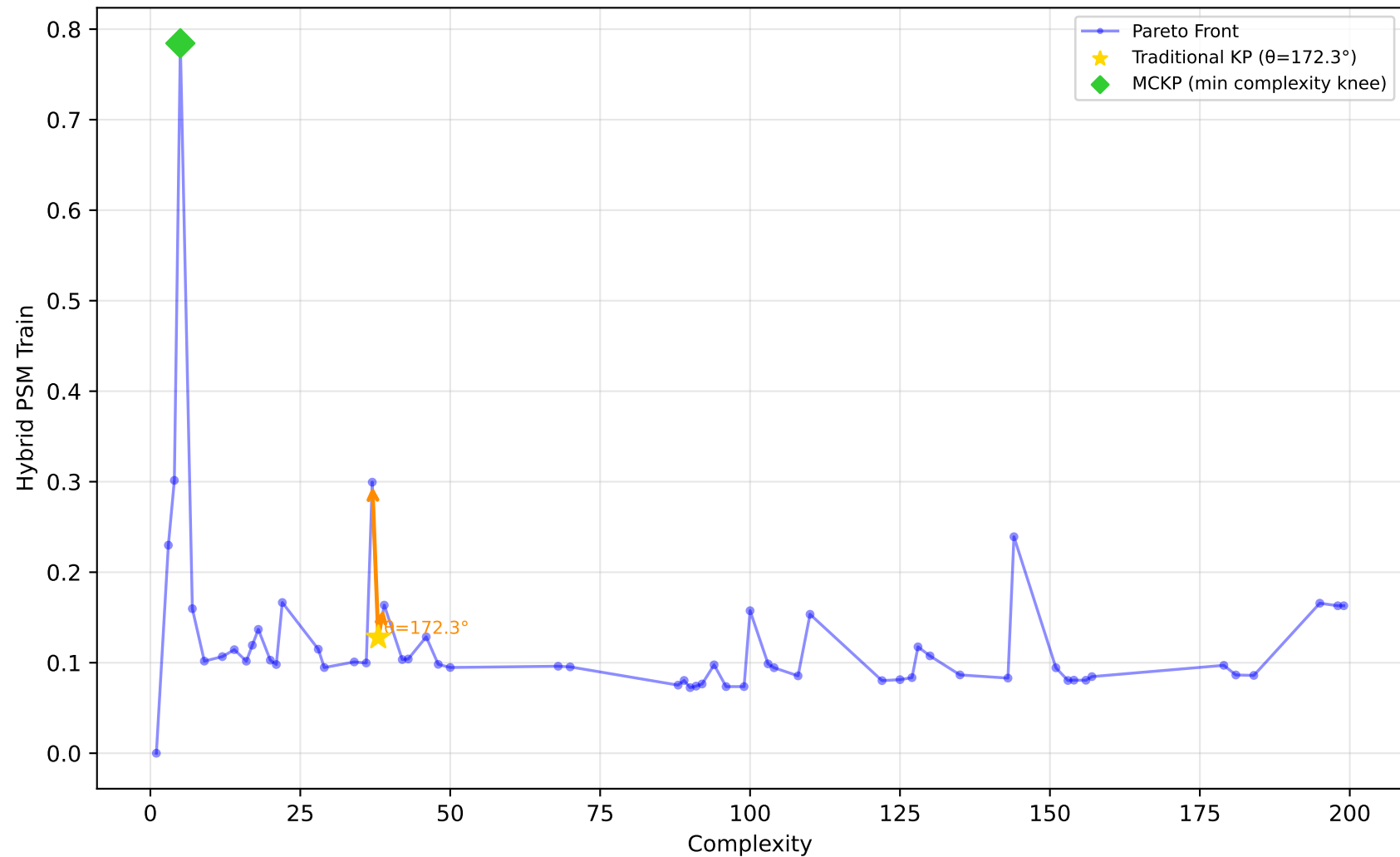
1096_FacultySalaries - Run 24 - MVP - Hybrid PSM Train \lambda_1=1.00, \lambda_2=0.00, \lambda_3=0.00 | Difficulty: 0.58 | Method: mckp
