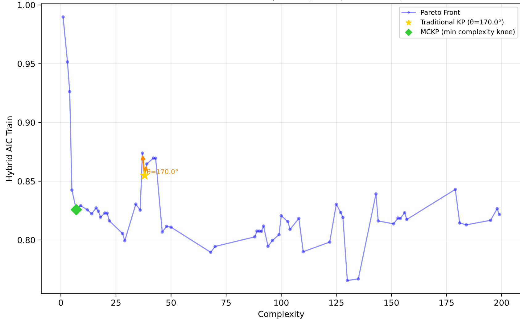
1096_FacultySalaries - Run 24 - SVP - Hybrid AIC Train \lambda_1=0.00, \lambda_2=0.90, \lambda_3=0.00 | Difficulty: 0.58 | Method: mckp
