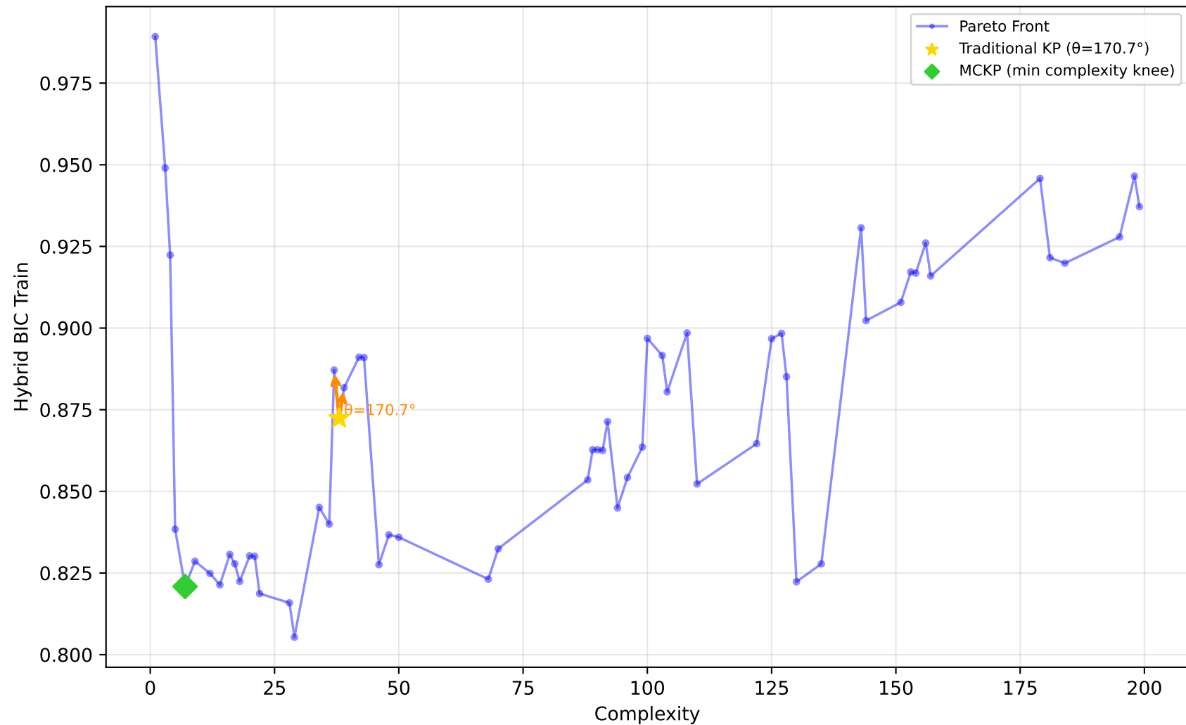
1096_FacultySalaries - Run 24 - SVP - Hybrid BIC Train \lambda_1=0.00, \lambda_2=0.90, \lambda_3=0.00 | Difficulty: 0.58 | Method: mckp
