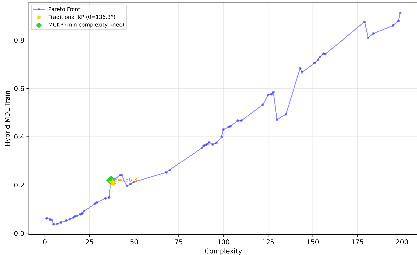
1096_FacultySalaries - Run 24 - SVP - Hybrid MDL Train \lambda_1=0.00 , \lambda_2=0.90 , \lambda_3=0.00 | Difficulty: 0.58 | Method: mckp
