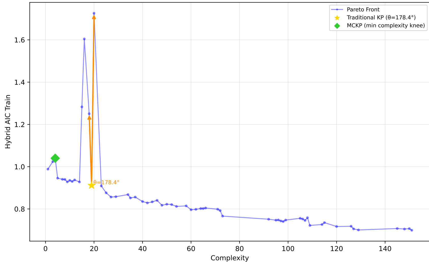
1096_FacultySalaries - Run 25 - MVP - Hybrid AIC Train \lambda_1=1.00 , \lambda_2=0.00 , \lambda_3=0.00 | Difficulty: 0.42 | Method: mckp
