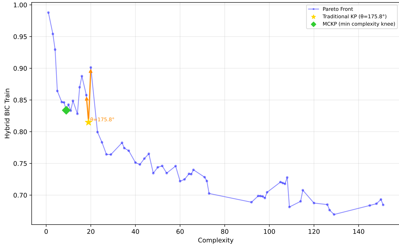
1096_FacultySalaries - Run 25 - MVP - Hybrid BIC Train \lambda_1=0.10 , \lambda_2=0.00 , \lambda_3=0.00 | Difficulty: 0.42 | Method: mckp
