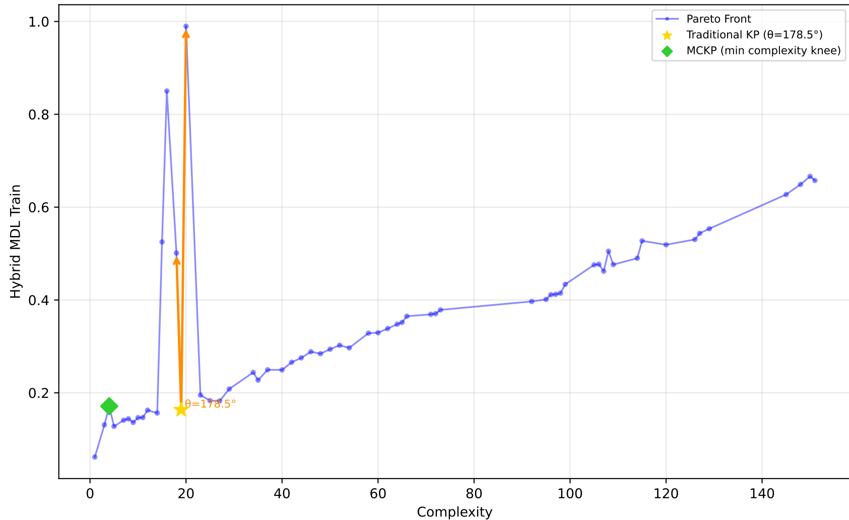
1096_FacultySalaries - Run 25 - MVP - Hybrid MDL Train \lambda_1=1.00 , \lambda_2=0.00 , \lambda_3=0.00 | Difficulty: 0.42 | Method: mckp
