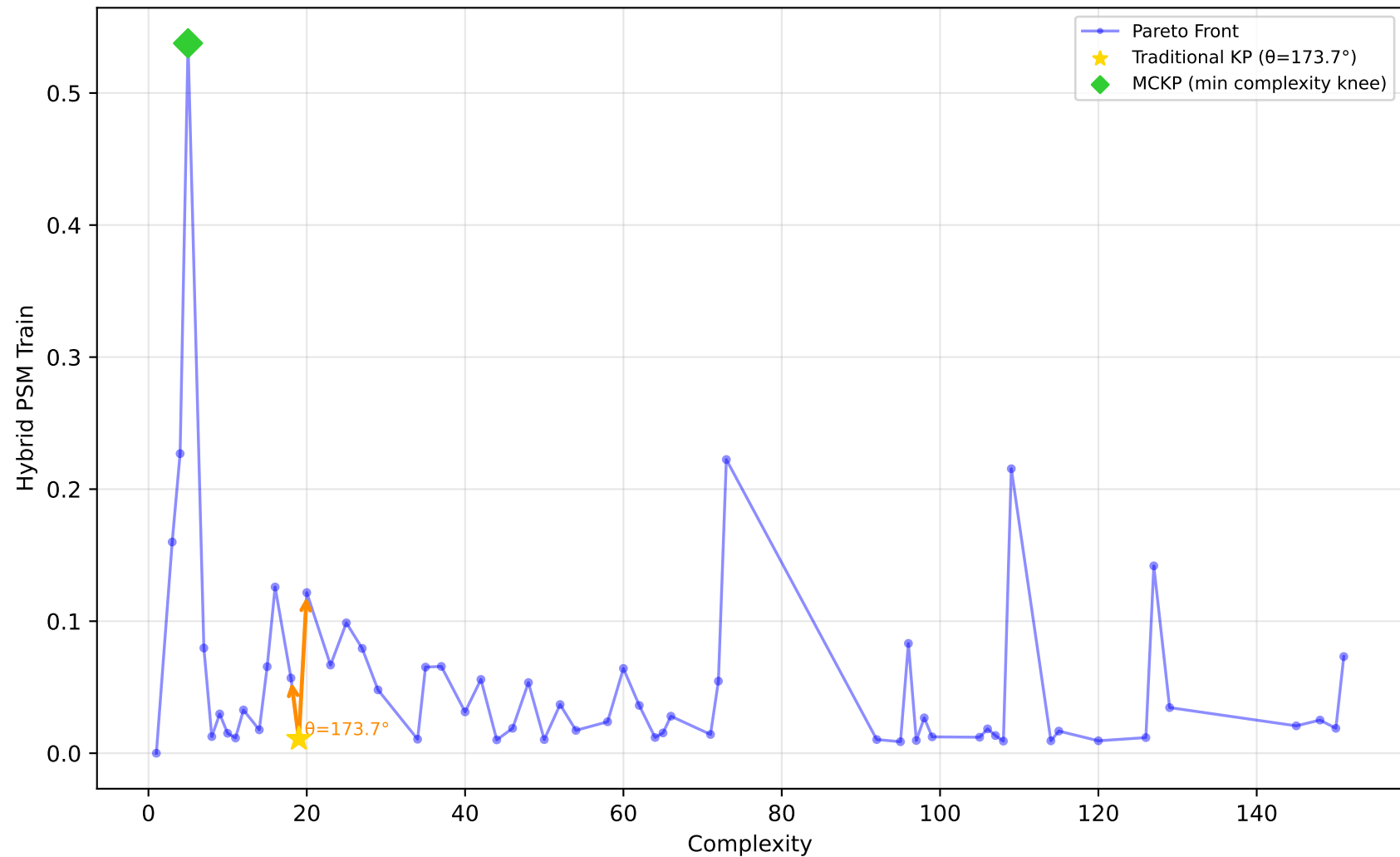
1096_FacultySalaries - Run 25 - MVP - Hybrid PSM Train \lambda_1=0.10, \lambda_2=0.00, \lambda_3=0.00 | Difficulty: 0.42 | Method: mckp
