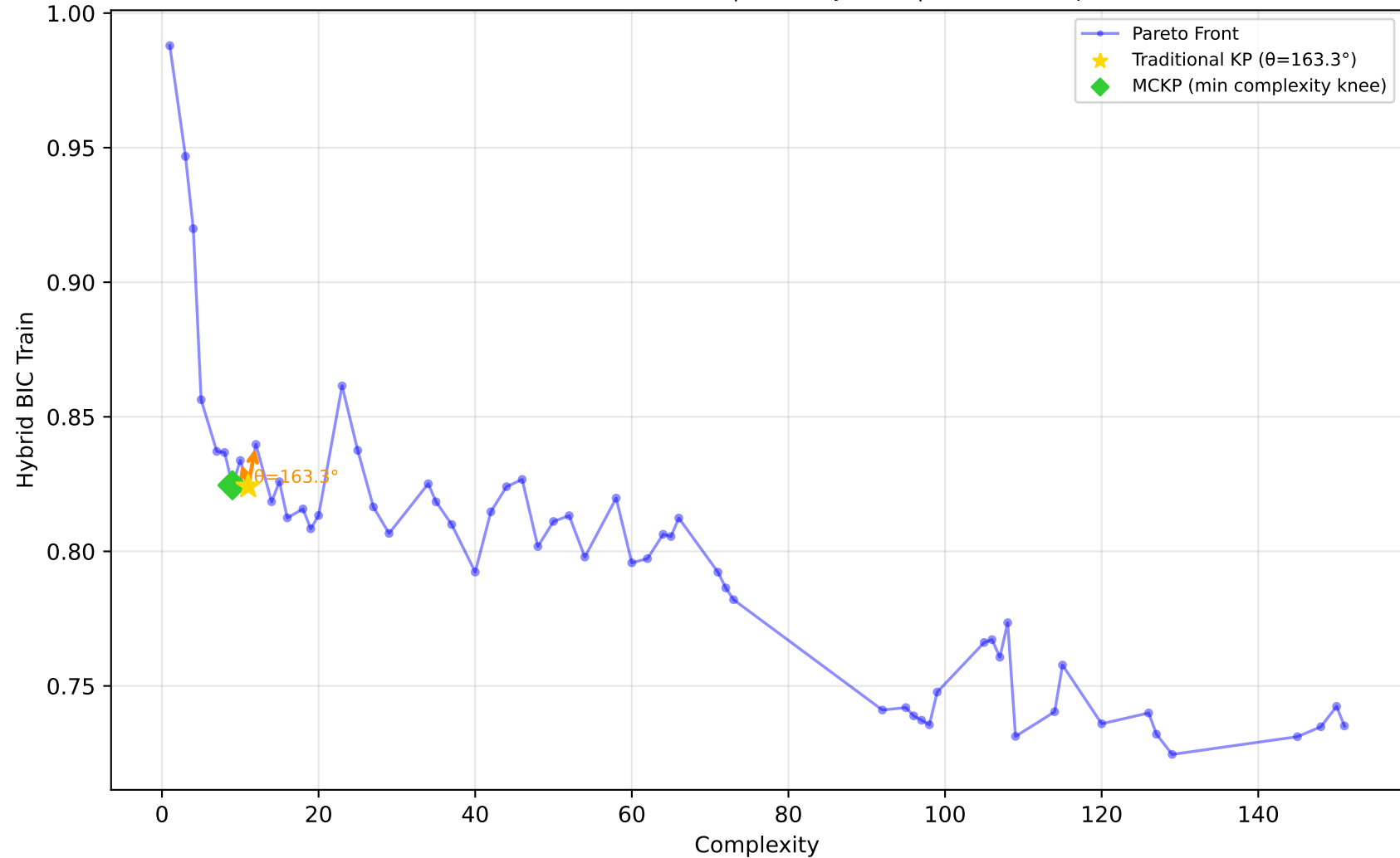
1096_FacultySalaries - Run 25 - SVP - Hybrid BIC Train \lambda_1=0.00, \lambda_2=0.90, \lambda_3=0.00 | Difficulty: 0.42 | Method: mckp
