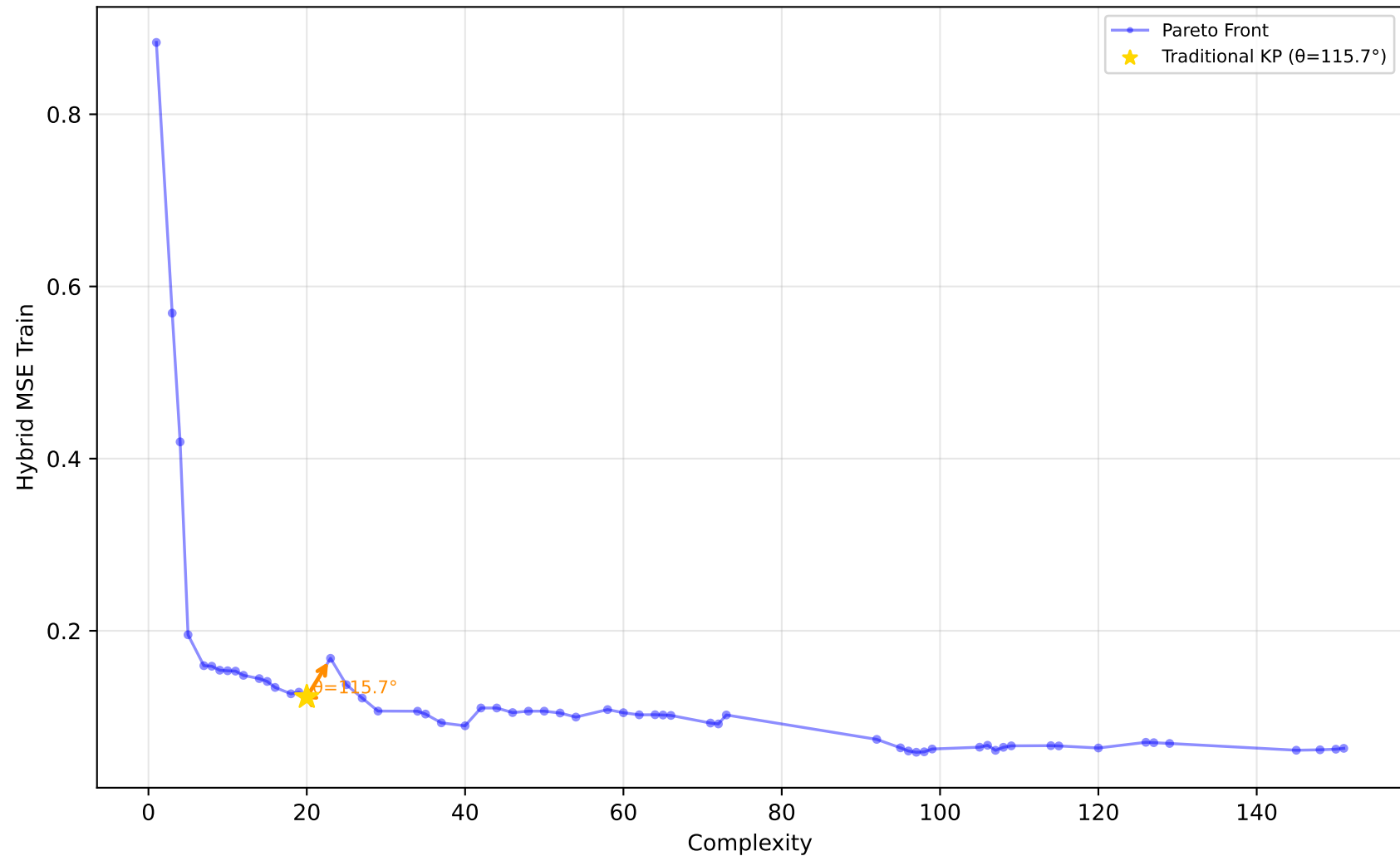
1096_FacultySalaries - Run 25 - SVP - Hybrid MSE Train \lambda_1=0.00, \lambda_2=0.90, \lambda_3=0.00 | Difficulty: 0.42 | Method: mckp
