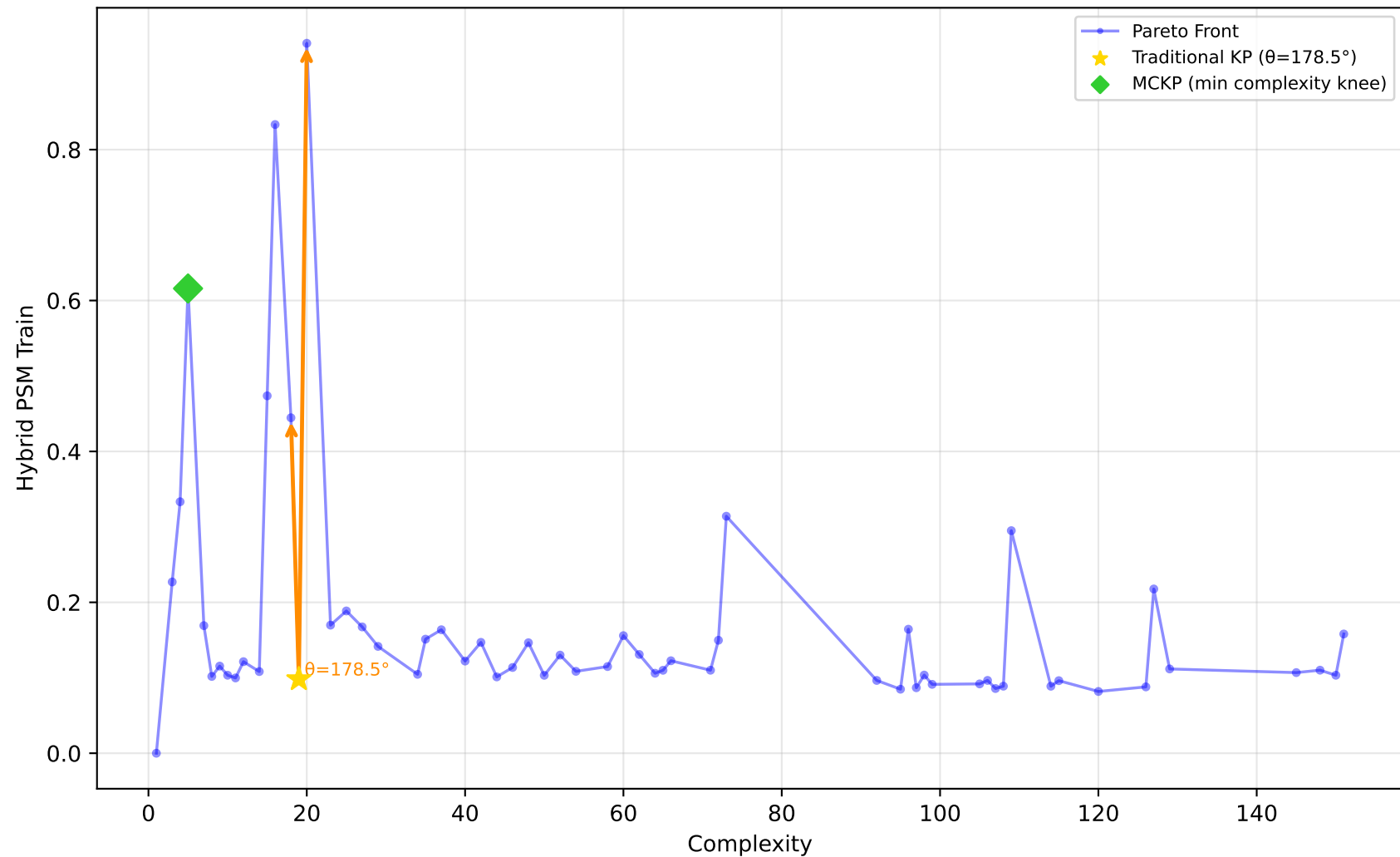
1096_FacultySalaries - Run 25 - SVP - Hybrid PSM Train \lambda_1=1.00, \lambda_2=0.00, \lambda_3=0.00 | Difficulty: 0.42 | Method: mckp
