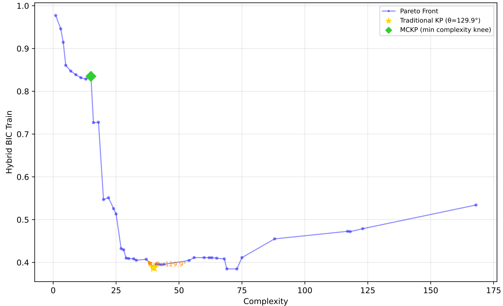
1096_FacultySalaries - Run 26 - MVP - Hybrid BIC Train \lambda_1=0.10 , \lambda_2=0.00 , \lambda_3=0.00 | Difficulty: 1.00 | Method: hmr
