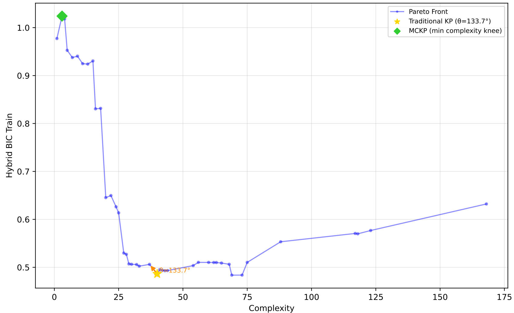
1096_FacultySalaries - Run 26 - MVP - Hybrid BIC Train \lambda_1=1.00 , \lambda_2=0.00 , \lambda_3=0.00 | Difficulty: 1.00 | Method: hmr
