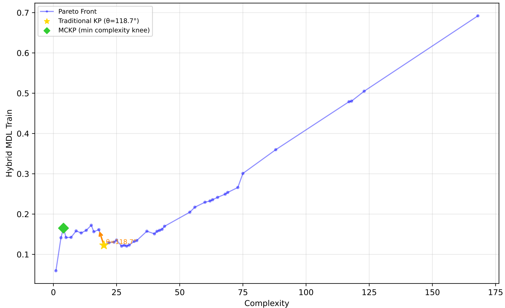
1096_FacultySalaries - Run 26 - MVP - Hybrid MDL Train \lambda_1=1.00 , \lambda_2=0.00 , \lambda_3=0.00 | Difficulty: 1.00 | Method: hmr
