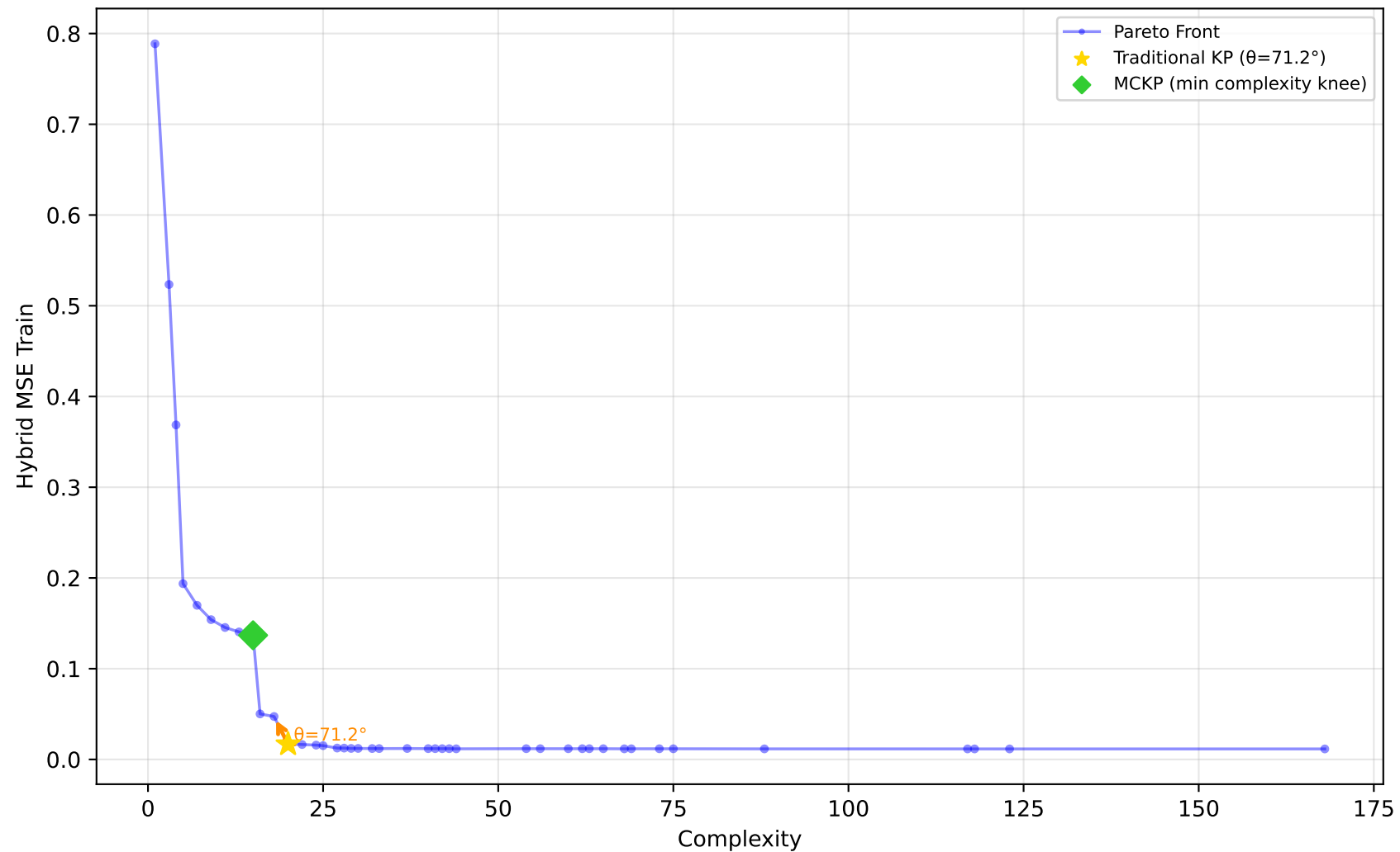
1096_FacultySalaries - Run 26 - MVP - Hybrid MSE Train \lambda_1=0.10 , \lambda_2=0.00 , \lambda_3=0.00 | Difficulty: 1.00 | Method: hmr
