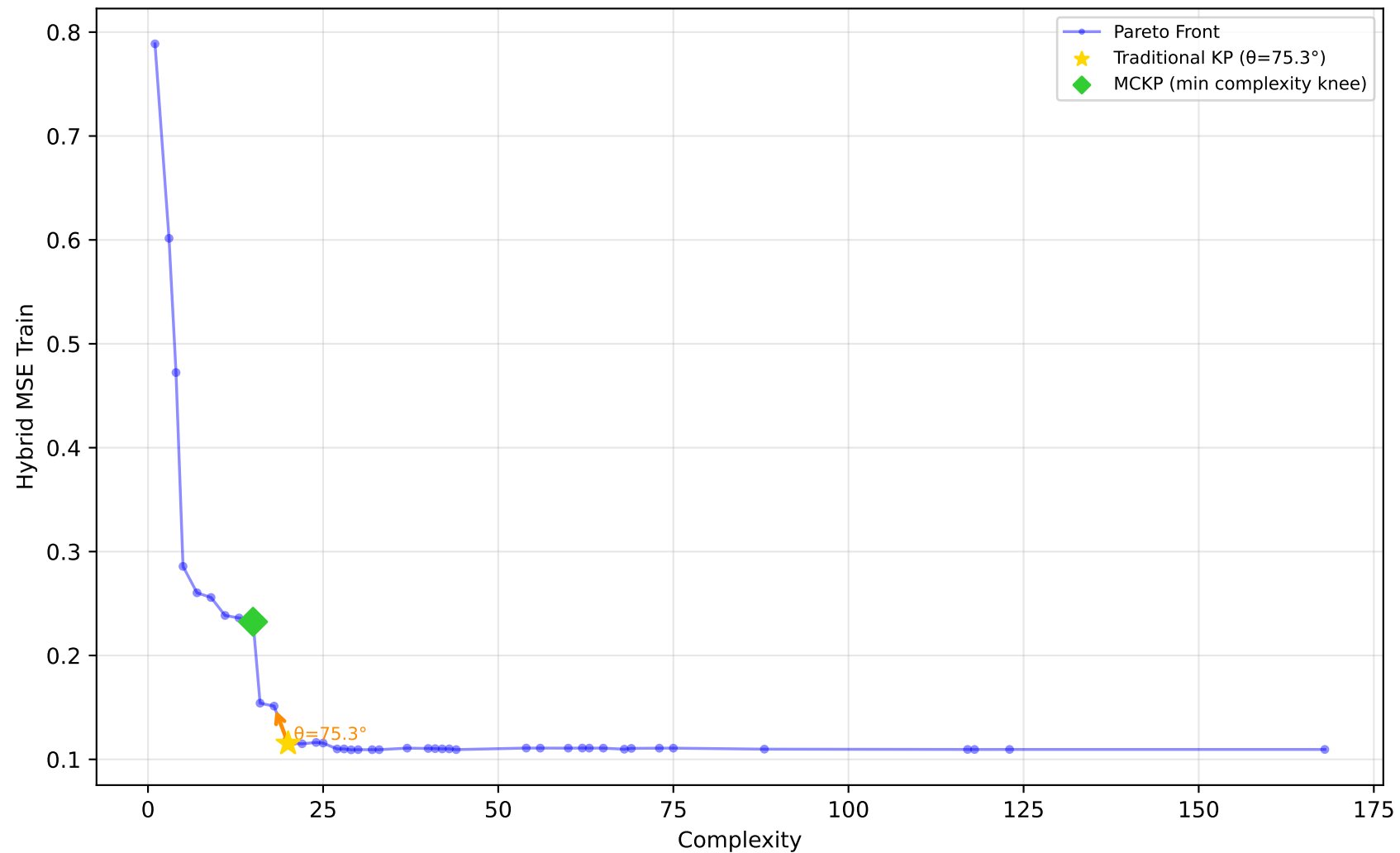
1096_FacultySalaries - Run 26 - MVP - Hybrid MSE Train \lambda_1=1.00 , \lambda_2=0.00 , \lambda_3=0.00 | Difficulty: 1.00 | Method: hmr
