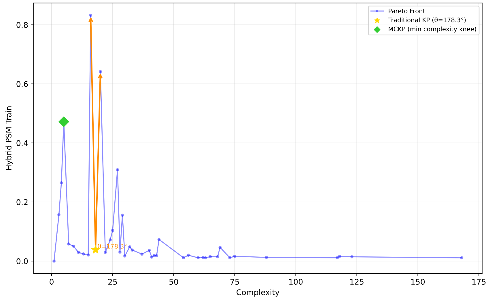
1096_FacultySalaries - Run 26 - MVP - Hybrid PSM Train \lambda_1=0.10 , \lambda_2=0.00 , \lambda_3=0.00 | Difficulty: 1.00 | Method: hmr
