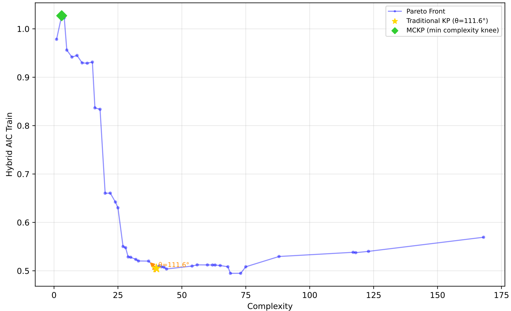
1096_FacultySalaries - Run 26 - SVP - Hybrid AIC Train \lambda_1=1.00 , \lambda_2=0.00 , \lambda_3=0.00 | Difficulty: 1.00 | Method: hmr
