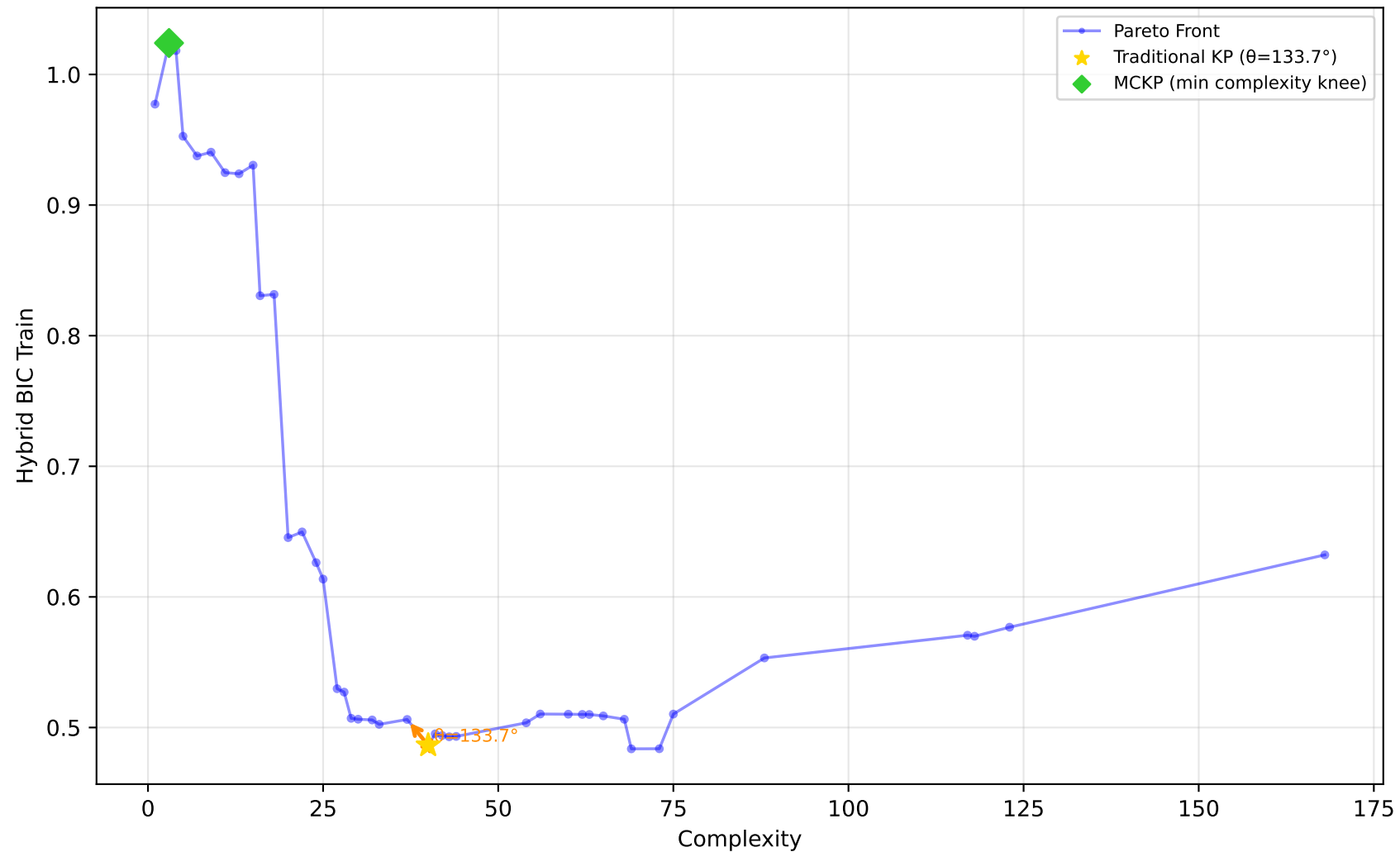
1096_FacultySalaries - Run 26 - SVP - Hybrid BIC Train \lambda_1=1.00 , \lambda_2=0.00 , \lambda_3=0.00 | Difficulty: 1.00 | Method: hmr
