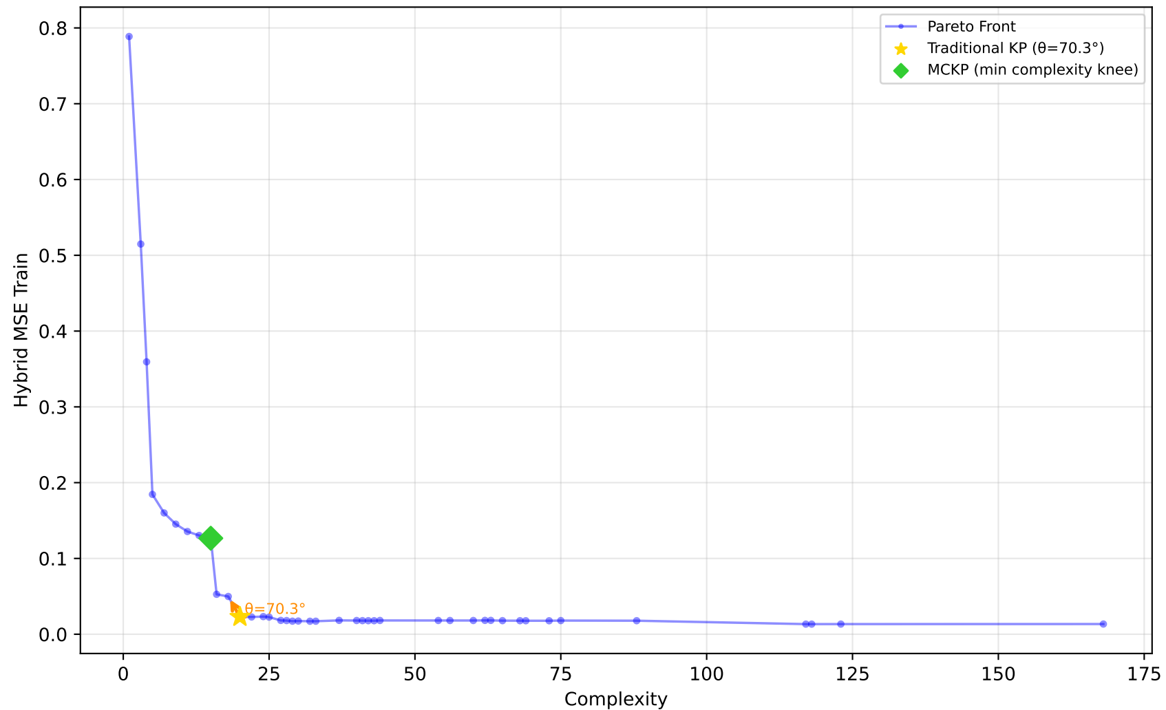
1096_FacultySalaries - Run 26 - SVP - Hybrid MSE Train \lambda_1=0.00 , \lambda_2=0.90 , \lambda_3=0.00 | Difficulty: 1.00 | Method: hmr
