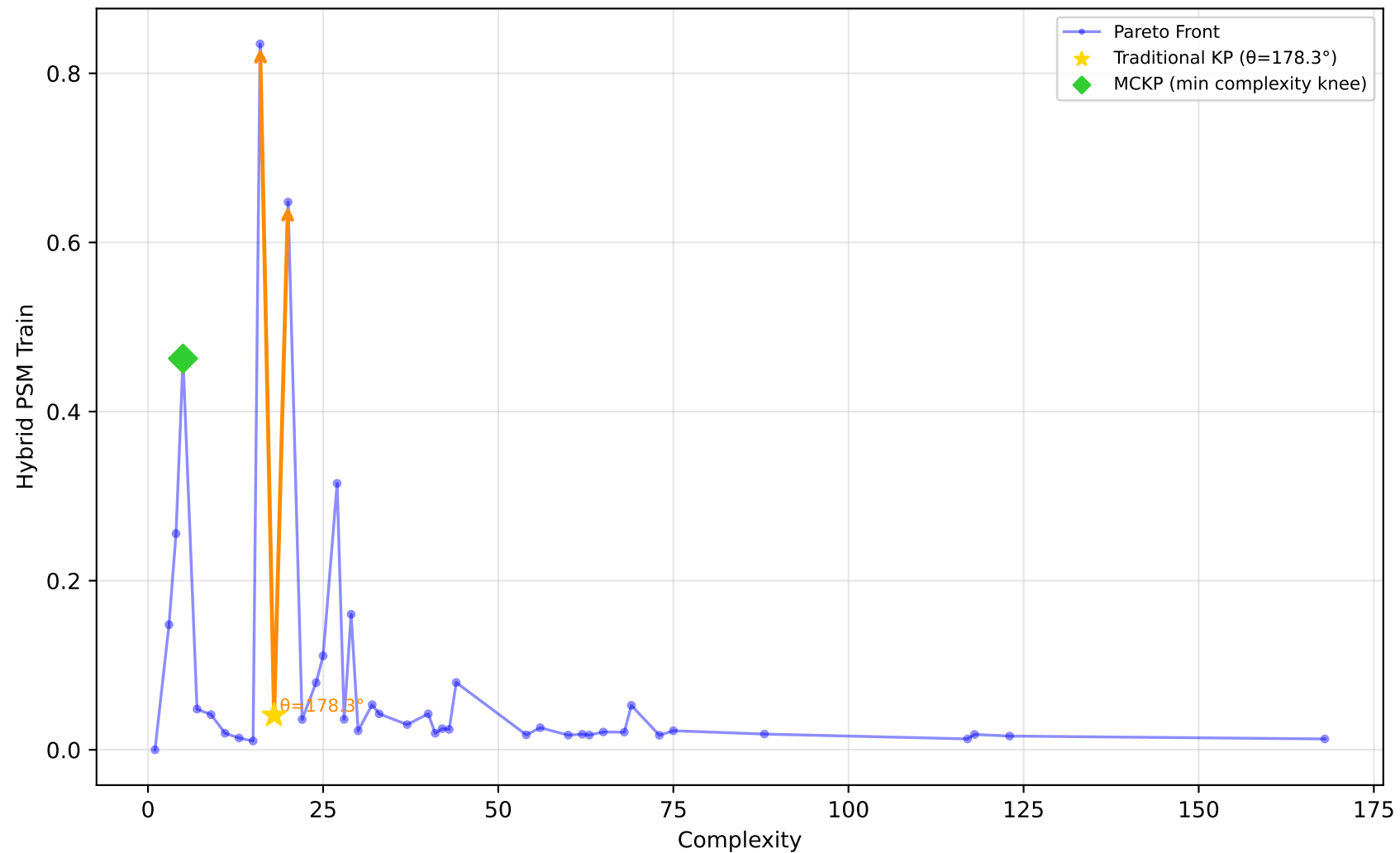
1096_FacultySalaries - Run 26 - SVP - Hybrid PSM Train \lambda_1=0.00, \lambda_2=0.90, \lambda_3=0.00 | Difficulty: 1.00 | Method: hmr
