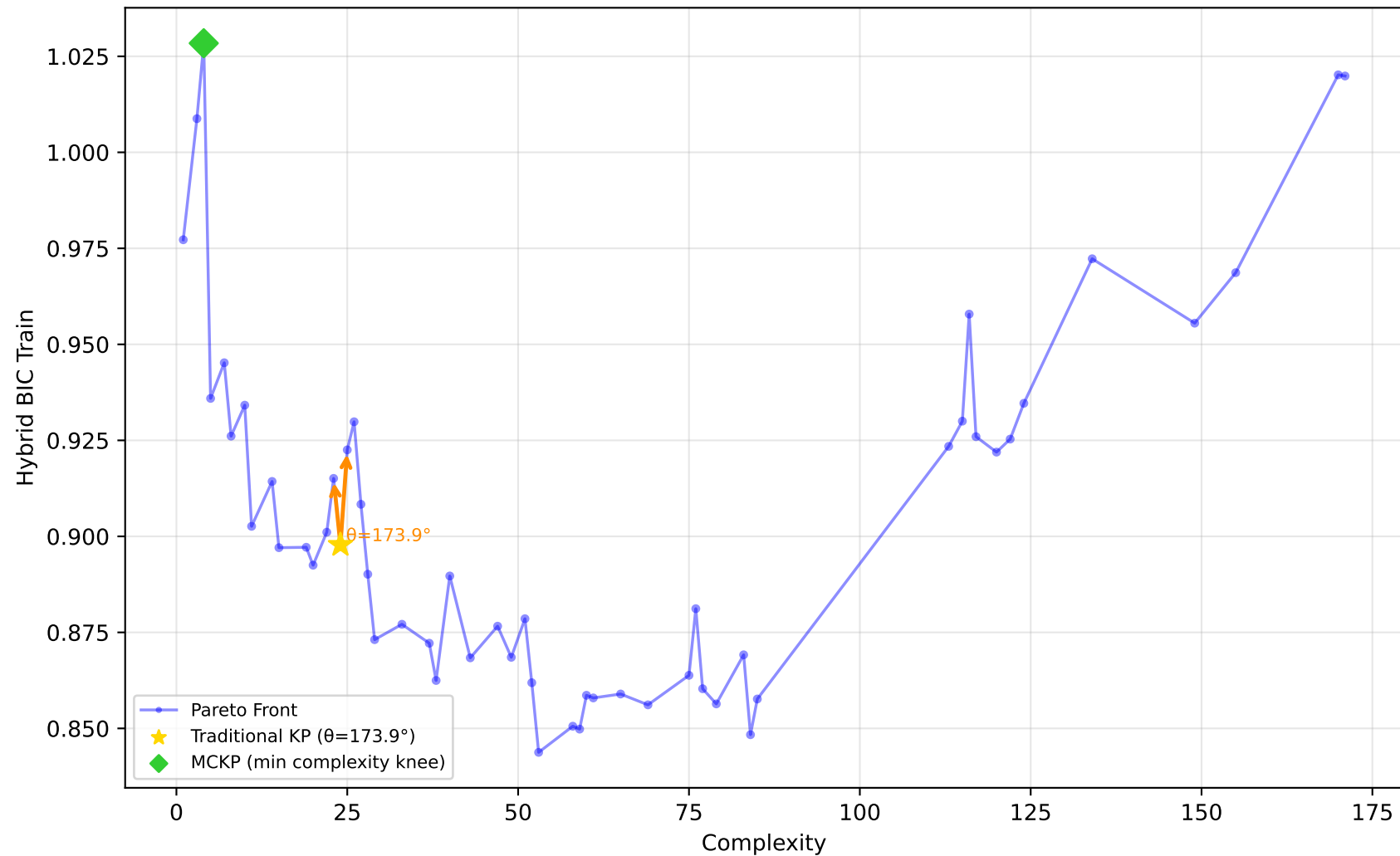
1096_FacultySalaries - Run 27 - MVP - Hybrid BIC Train \lambda_1=1.00 , \lambda_2=0.00 , \lambda_3=0.00 | Difficulty: 0.84 | Method: hmr
