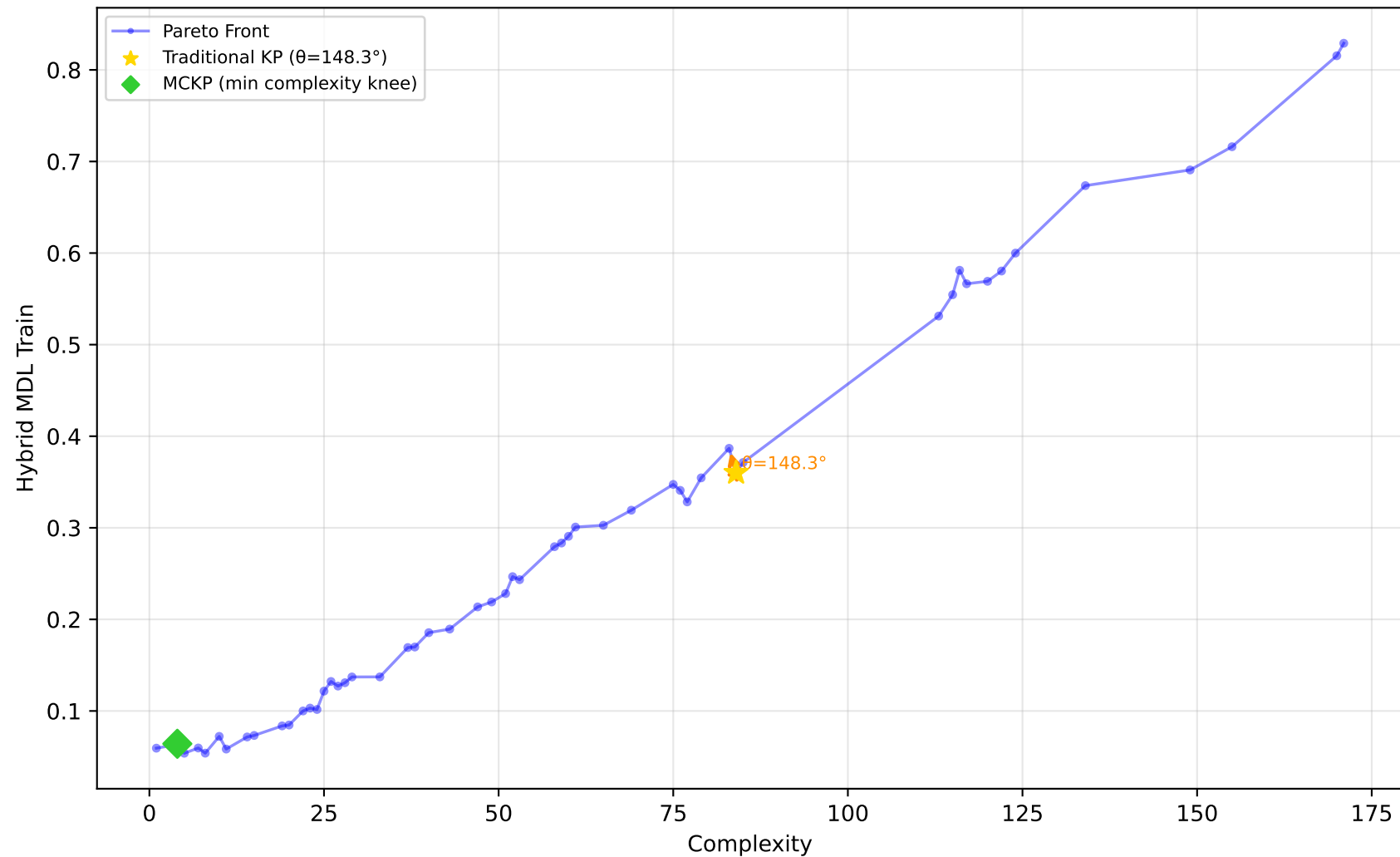
1096_FacultySalaries - Run 27 - MVP - Hybrid MDL Train \lambda_1=0.10 , \lambda_2=0.00 , \lambda_3=0.00 | Difficulty: 0.84 | Method: hmr
