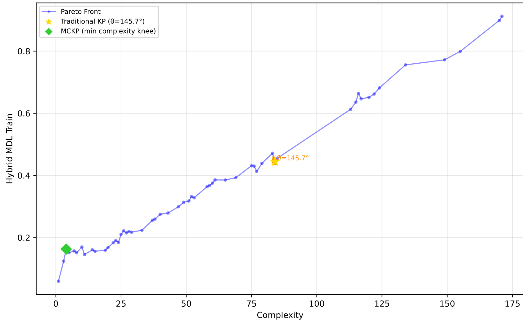
1096_FacultySalaries - Run 27 - MVP - Hybrid MDL Train \lambda_1=1.00 , \lambda_2=0.00 , \lambda_3=0.00 | Difficulty: 0.84 | Method: hmr
