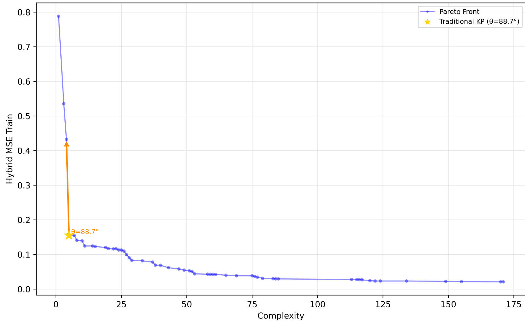
1096_FacultySalaries - Run 27 - MVP - Hybrid MSE Train \lambda_1=0.10, \lambda_2=0.00, \lambda_3=0.00 | Difficulty: 0.84 | Method: hmr
