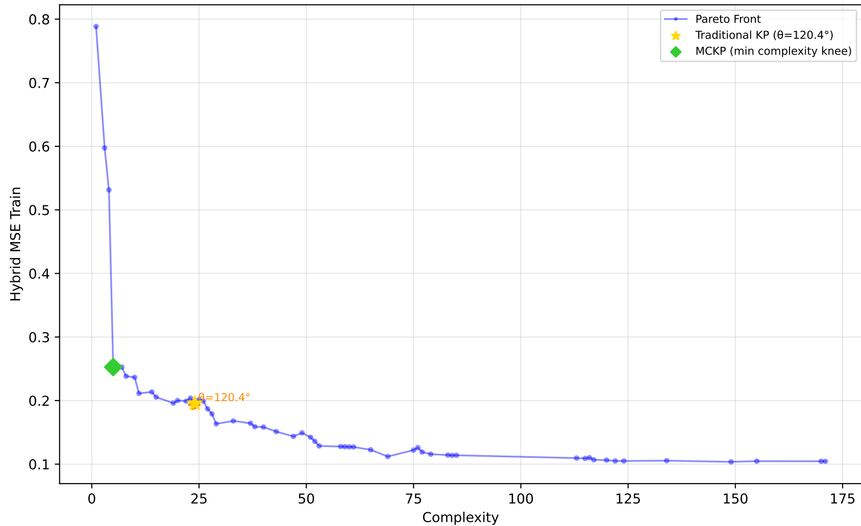
1096_FacultySalaries - Run 27 - MVP - Hybrid MSE Train \lambda_1=1.00 , \lambda_2=0.00 , \lambda_3=0.00 | Difficulty: 0.84 | Method: hmr
