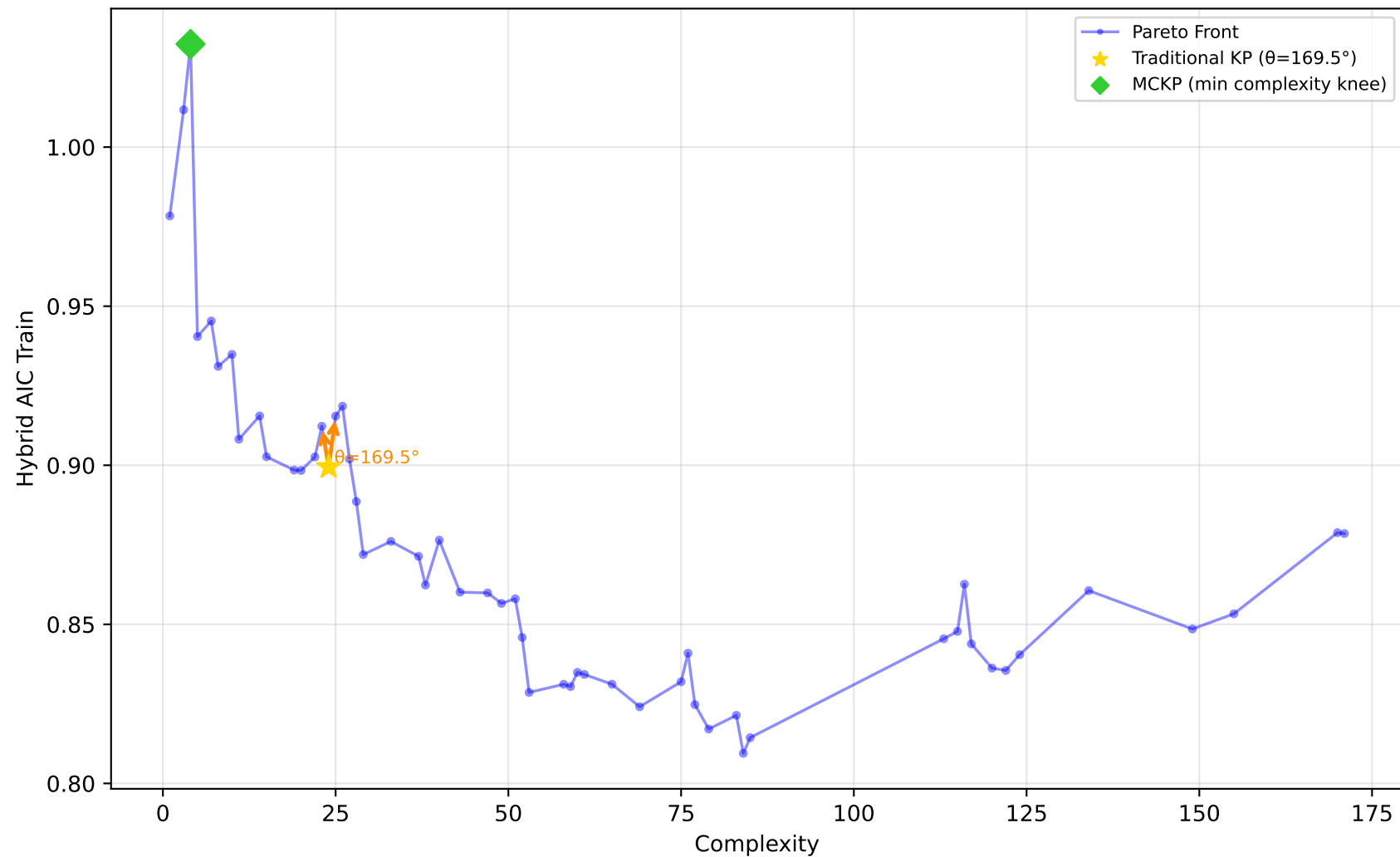
1096_FacultySalaries - Run 27 - SVP - Hybrid AIC Train \lambda_1=1.00 , \lambda_2=0.00 , \lambda_3=0.00 | Difficulty: 0.84 | Method: hmr
