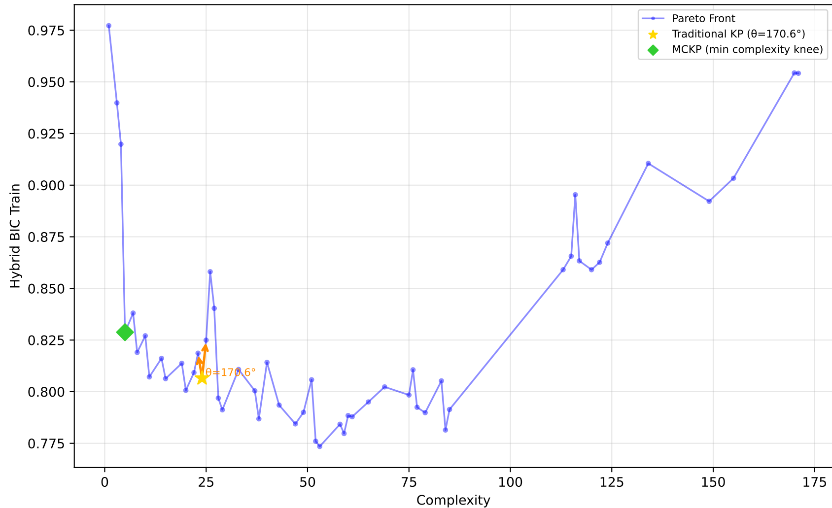
1096_FacultySalaries - Run 27 - SVP - Hybrid BIC Train \lambda_1=0.00, \lambda_2=0.90, \lambda_3=0.00 | Difficulty: 0.84 | Method: hmr
