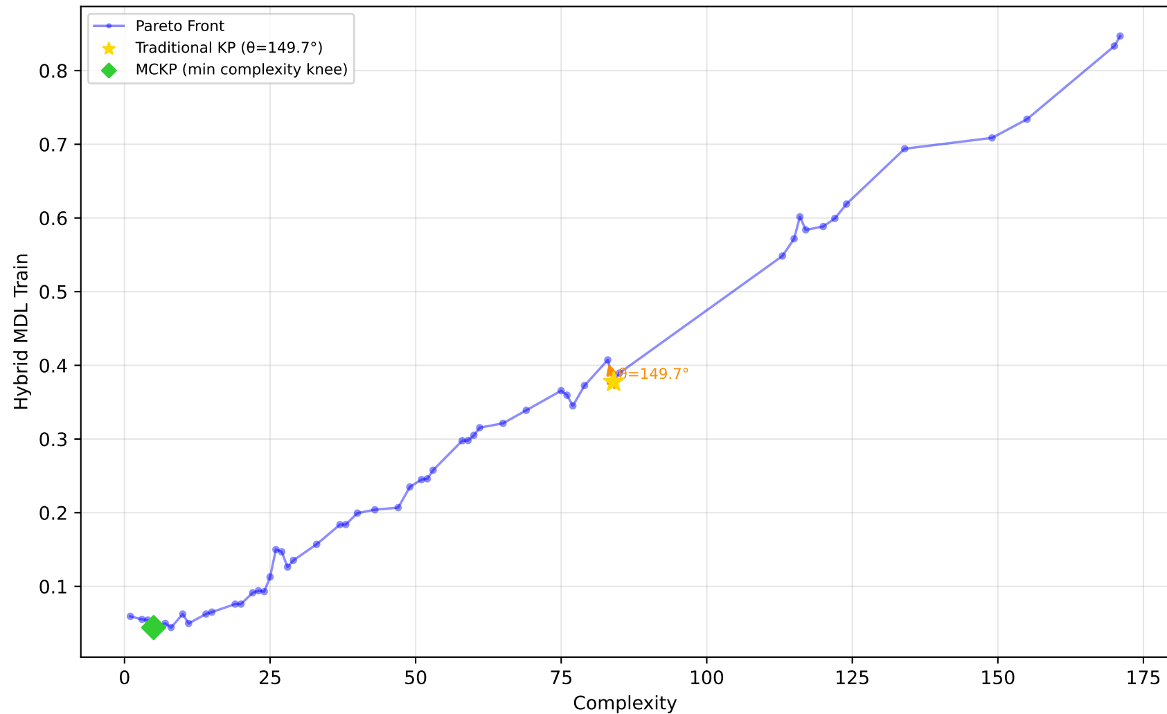
1096_FacultySalaries - Run 27 - SVP - Hybrid MDL Train \lambda_1=0.00 , \lambda_2=0.90 , \lambda_3=0.00 | Difficulty: 0.84 | Method: hmr
