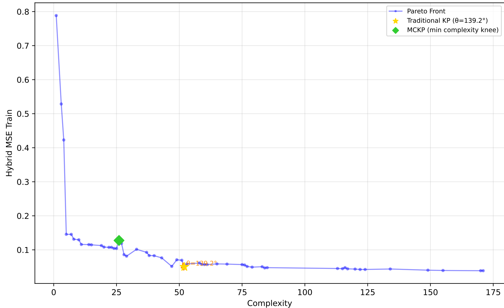
1096_FacultySalaries - Run 27 - SVP - Hybrid MSE Train \lambda_1=0.00, \lambda_2=0.90, \lambda_3=0.00 | Difficulty: 0.84 | Method: hmr
