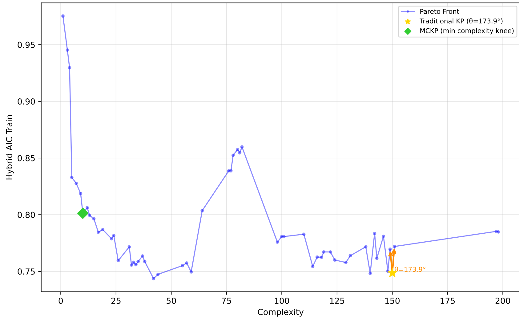
1096_FacultySalaries - Run 28 - MVP - Hybrid AIC Train \lambda_1=0.10 , \lambda_2=0.00 , \lambda_3=0.00 | Difficulty: 0.51 | Method: mckp
