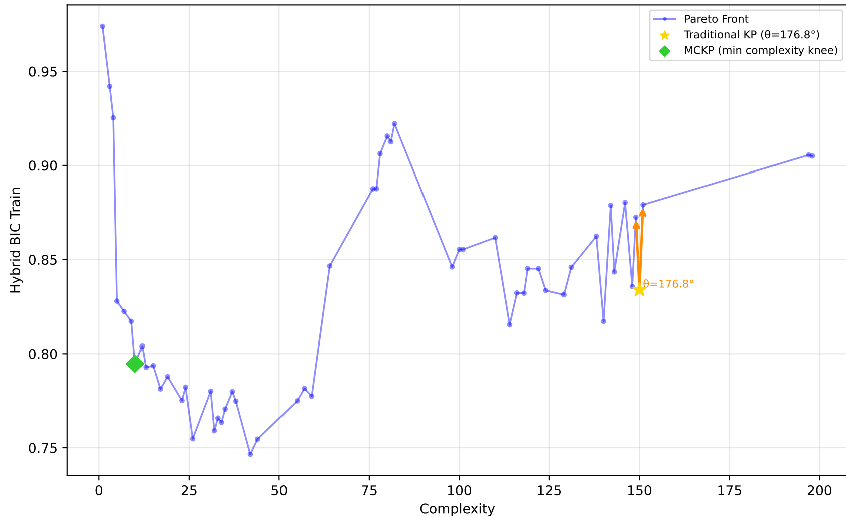
1096_FacultySalaries - Run 28 - MVP - Hybrid BIC Train \lambda_1=0.10, \lambda_2=0.00, \lambda_3=0.00 | Difficulty: 0.51 | Method: mckp
