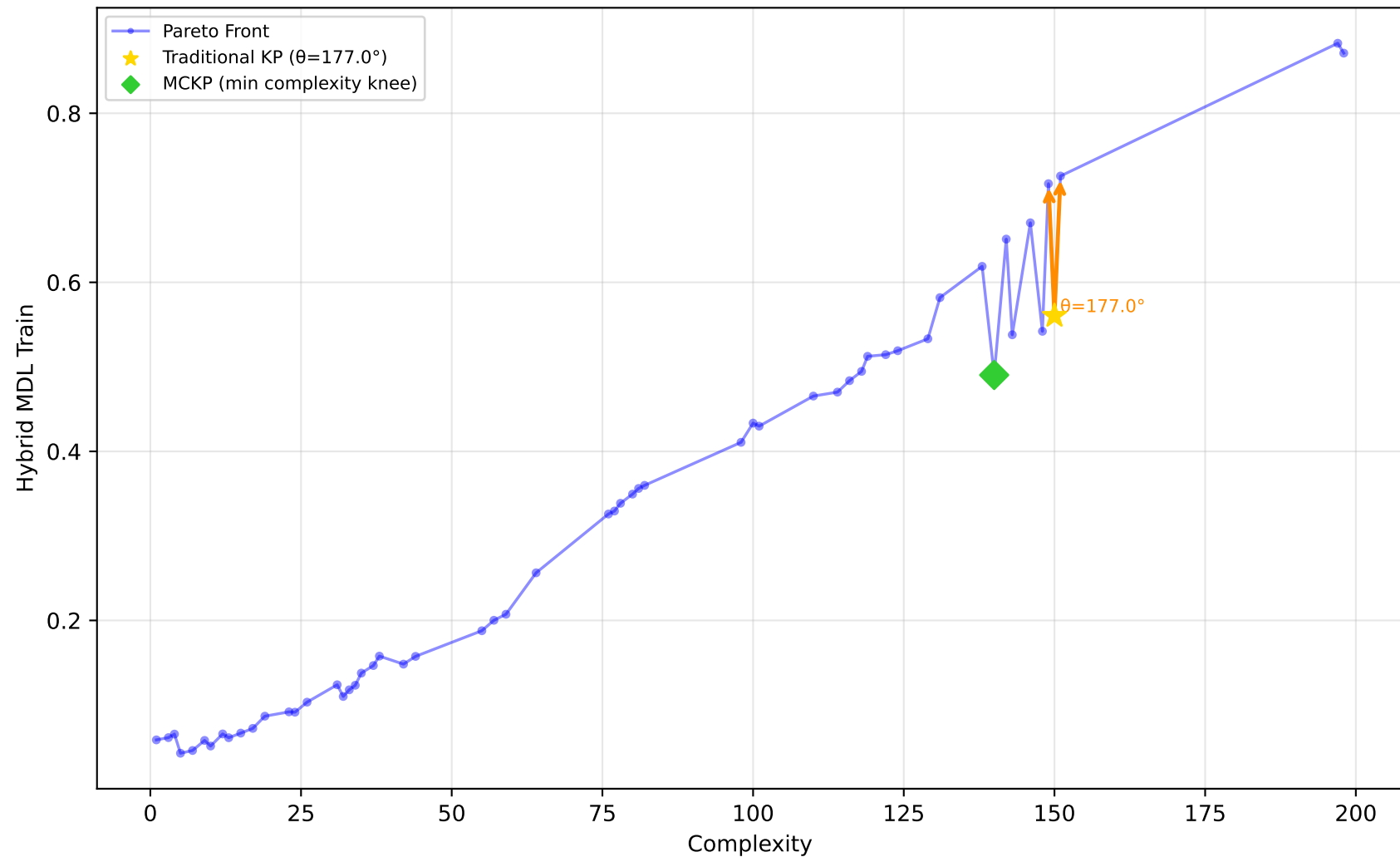
1096_FacultySalaries - Run 28 - MVP - Hybrid MDL Train \lambda_1=0.10, \lambda_2=0.00, \lambda_3=0.00 | Difficulty: 0.51 | Method: mckp
