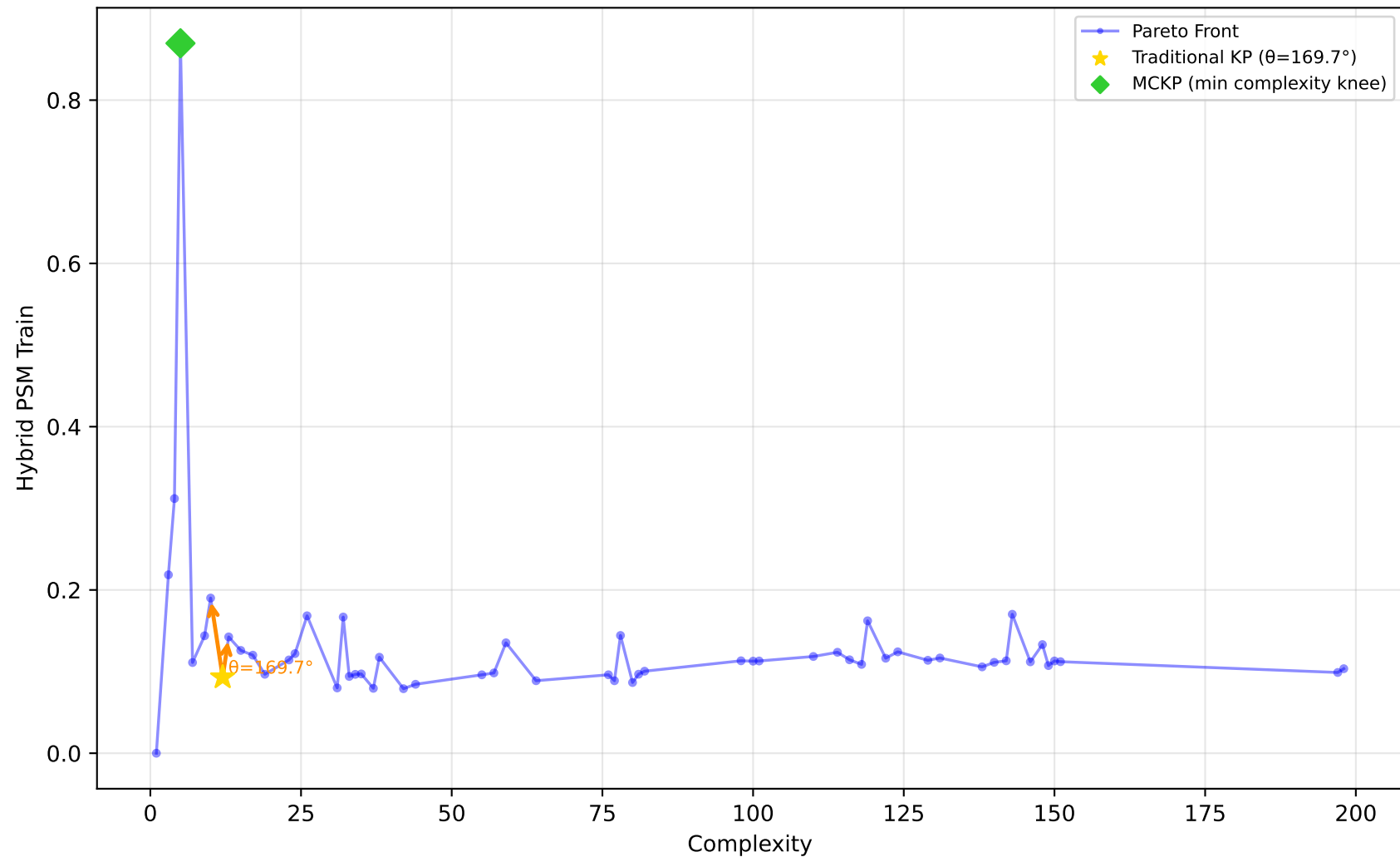
1096_FacultySalaries - Run 28 - MVP - Hybrid PSM Train \lambda_1=1.00, \lambda_2=0.00, \lambda_3=0.00 | Difficulty: 0.51 | Method: mckp
