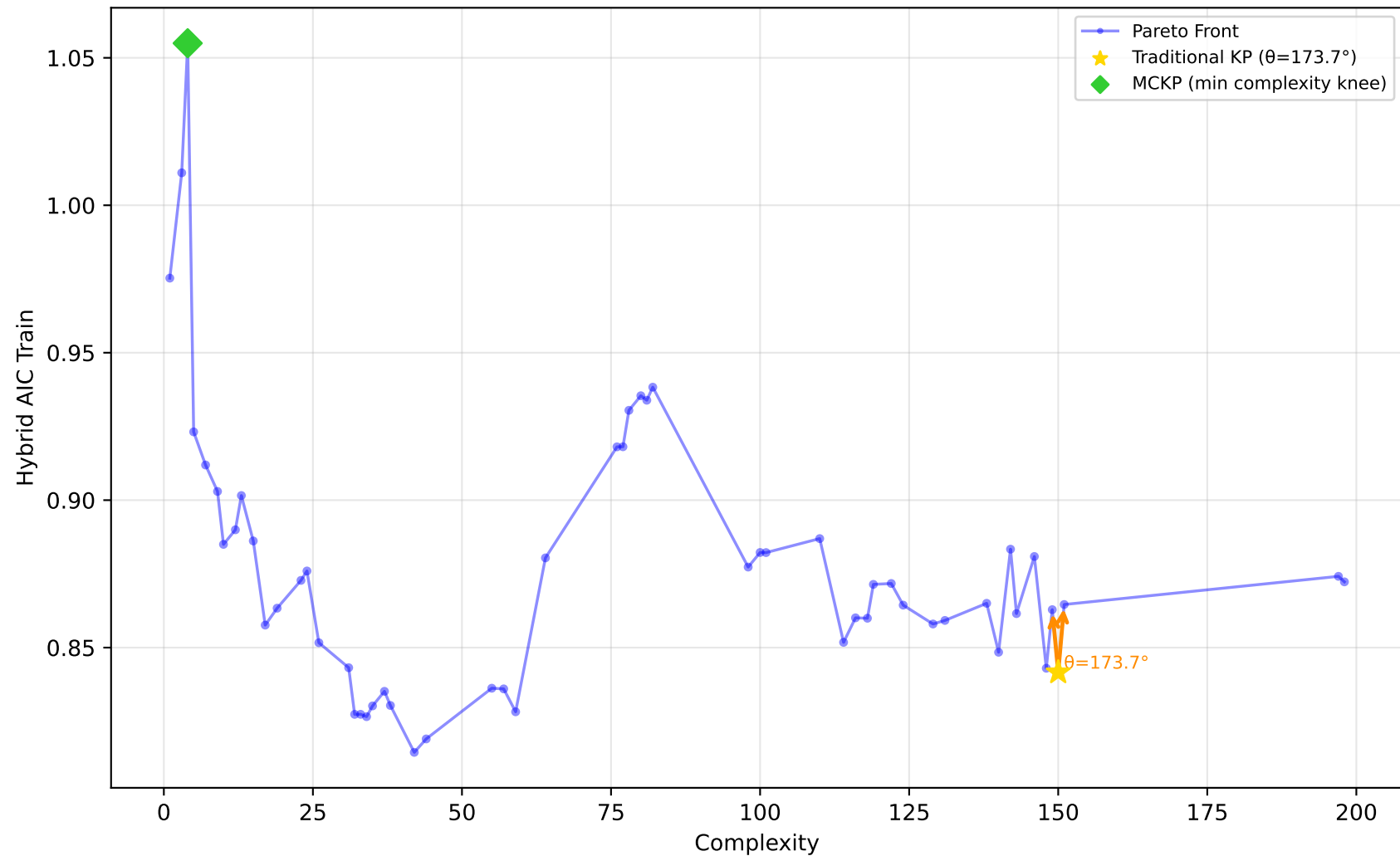
1096_FacultySalaries - Run 28 - SVP - Hybrid AIC Train \lambda_1=1.00, \lambda_2=0.00, \lambda_3=0.00 | Difficulty: 0.51 | Method: mckp
