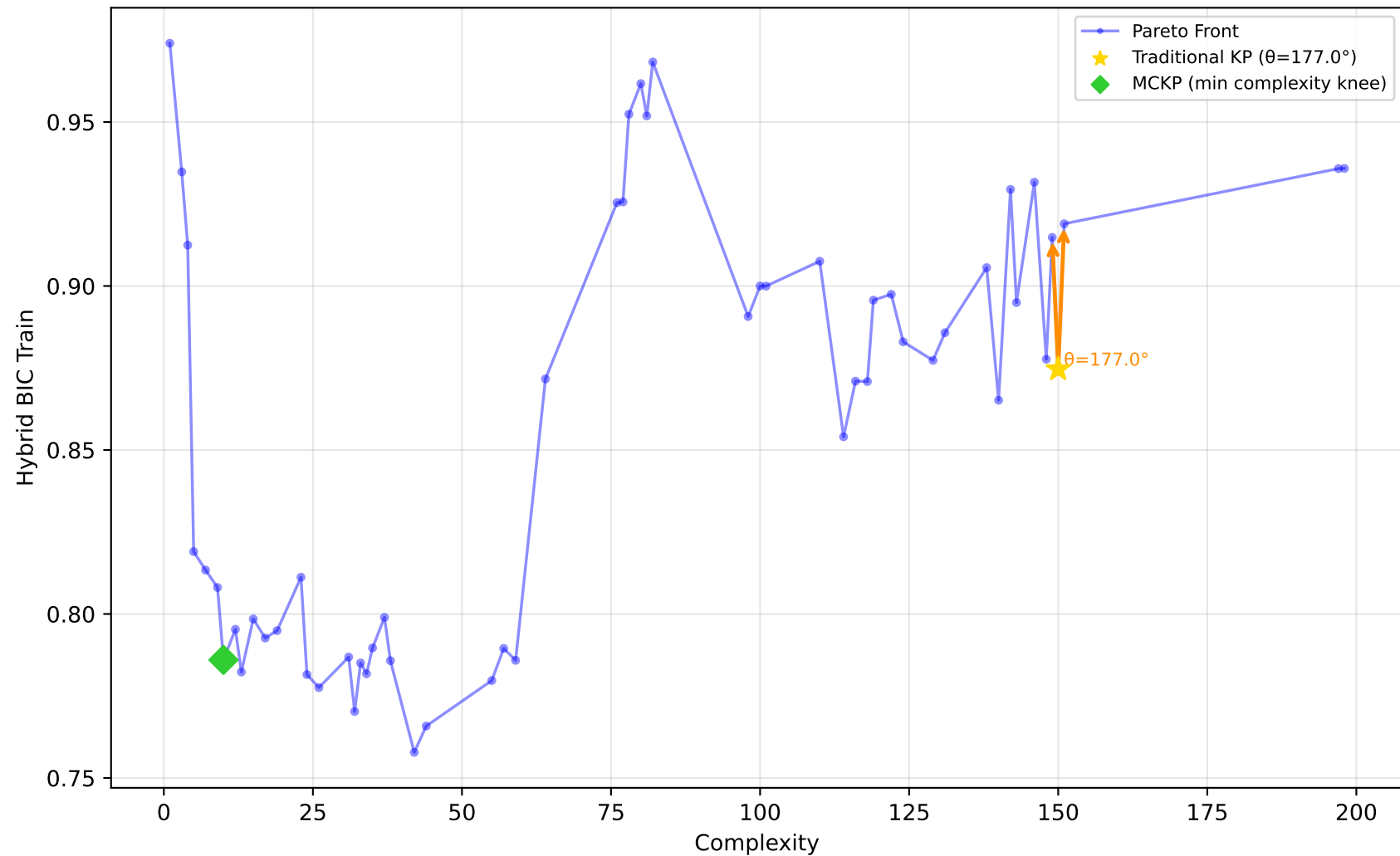
1096_FacultySalaries - Run 28 - SVP - Hybrid BIC Train \lambda_1=0.00, \lambda_2=0.90, \lambda_3=0.00 | Difficulty: 0.51 | Method: mckp
