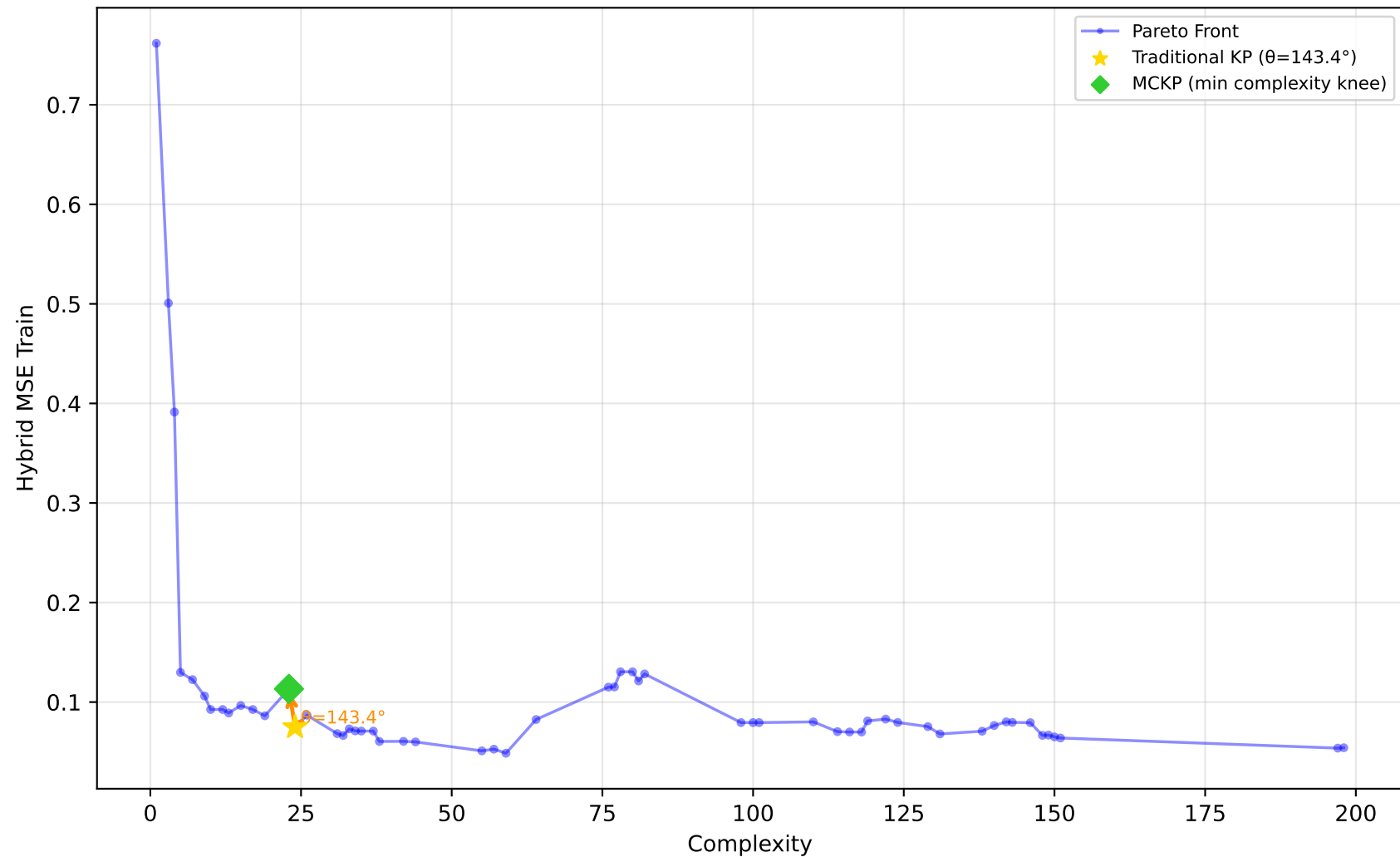
1096_FacultySalaries - Run 28 - SVP - Hybrid MSE Train \lambda_1=0.00, \lambda_2=0.90, \lambda_3=0.00 | Difficulty: 0.51 | Method: mckp
